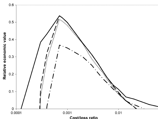
FIGURE 6 Value plot with a log scale x -axis of the global turbulence forecast performance with the 98 convective turbulence cases removed showing the forecast value of the Met Office Global and Regional Ensemble Prediction System (dot-dashed), the European Centre for Medium-Range Weather Forecasts Ensemble Prediction System (dotted), the combined multi-model ensemble (dashed) and the maximum value using every threshold of the combined multi-model ensemble (solid line). The data used have a forecast lead time between +24 hr and +33 hr between May 2016 and April 2017
