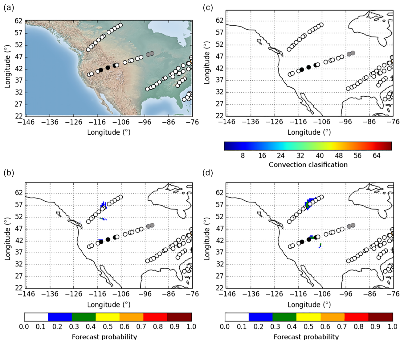
FIGURE 4 Plot of a moderate or greater turbulence event over the possible sources of turbulence: (a) orography, shear turbulence (b) Met Office Global and Regional Ensemble Prediction System and (d) European Centre for Medium-Range Weather Forecasts Ensemble Prediction System [ECMWF EPS] probability forecast) and (c) convection from satellite data. Only the ECMWF EPS ensemble forecasts the shear turbulence event. The circles indicate turbulence observations with white indicating no turbulence, grey indicating light turbulence and black indicating moderate or greater turbulence. The convective classification can be found in Francis and Batstone (2013) [Colour figure can be viewed at wileyonlinelibrary.com ]
