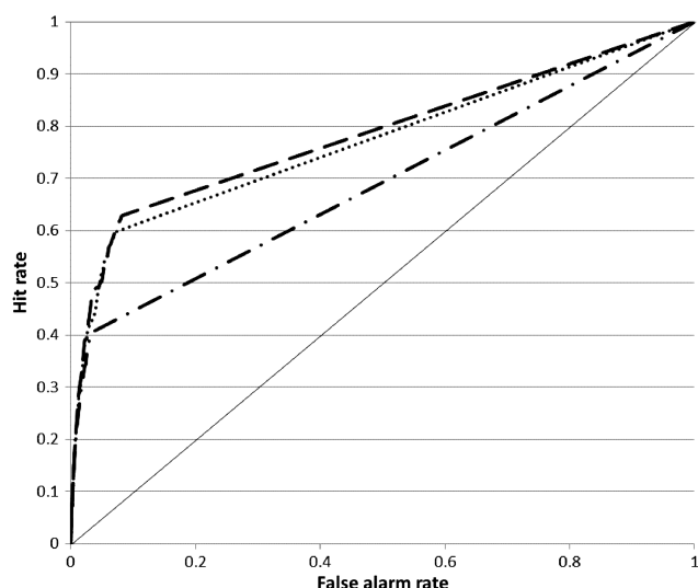
FIGURE 5 Relative operating characteristic plot of the global turbulence forecast performance with the 98 convective turbulence cases removed showing the forecast skill of the Met Office Global and Regional Ensemble Prediction System (dot-dashed) area under the curve (AUC) = 0.6881, the European Centre for Medium-Range Weather Forecasts Ensemble Prediction System (dotted) AUC = 0.772 and the combined multi-model ensemble (dashed) AUC = 0.7842. The data used have a forecast lead time between +24 hr and +33 hr between May 2016 and April 2017
