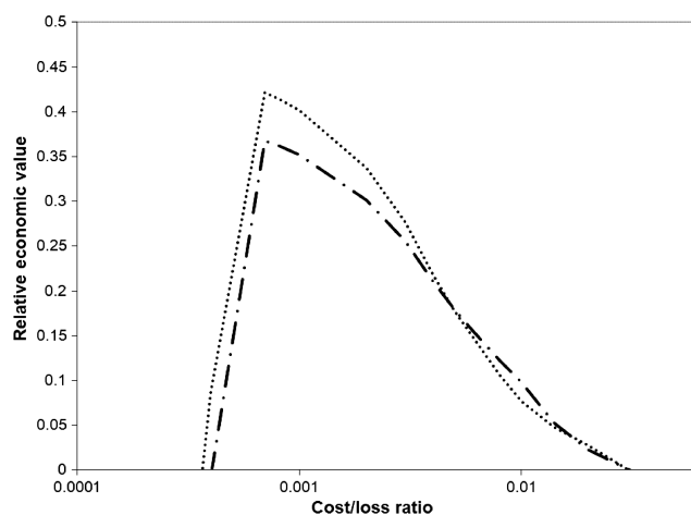
FIGURE 9 Value plot with a log scale x -axis of the global turbulence forecast performance showing the forecast value of the Met Office Global and Regional Ensemble Prediction System (dot-dashed) and the European Centre for Medium-Range Weather Forecasts 12 member ensemble (dotted). The data used have a forecast lead time between +24 hr and +33 hr between May 2016 and April 2017
