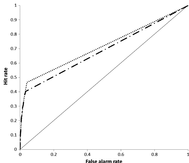
FIGURE 8 Relative operating characteristic plot of the global turbulence forecast performance showing the forecast skill of the Met Office Global and Regional Ensemble Prediction System (dot-dashed) and the European Centre for Medium-Range Weather Forecasts 12 member ensemble (dotted). The data used have a forecast lead time between +24 hr and +33 hr between May 2016 and April 2017
