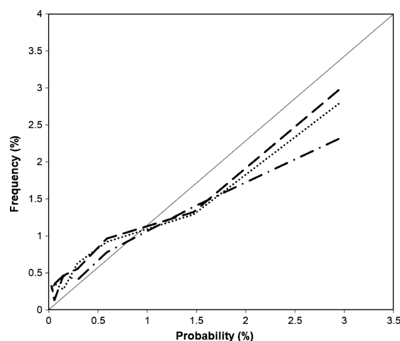
FIGURE 7 Reliability diagram of the Met Office Global and Regional Ensemble Prediction System (dot-dashed), the European Centre for Medium-Range Weather Forecasts Ensemble Prediction System (dotted) and the combined multi-model ensemble (dashed). The data used have a forecast lead time between +24 hr and +33 hr between May 2016 and April 2017
