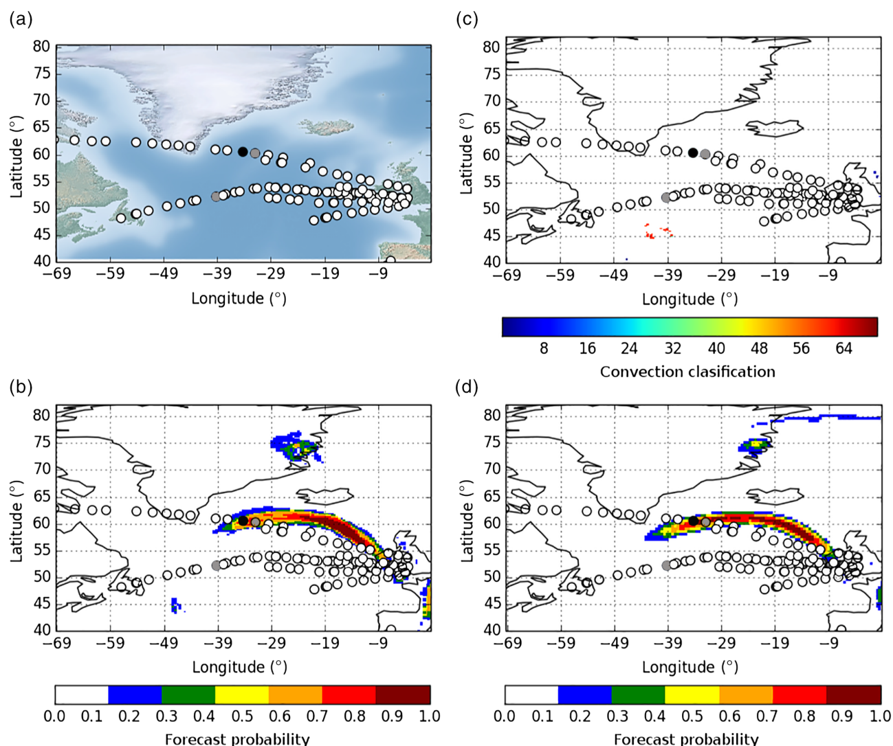
FIGURE 2 Plot of a moderate or greater turbulence event over the possible sources of turbulence: (a) orography, shear turbulence (b) Met Office Global and Regional Ensemble Prediction System [MOGREPS-G] and (d) European Centre for Medium-Range Weather Forecasts Ensemble Prediction System [ECMWF EPS] probability forecast) and (c) convection from satellite data. Both the MOGREPS-G and ECMWF EPS ensembles forecast the shear turbulence event. The circles indicate turbulence observations with white indicating no turbulence, grey indicating light turbulence and black indicating moderate or greater turbulence. The convective classification can be found in Francis and Batstone (2013) [Colour figure can be viewed at wileyonlinelibrary.com ]
