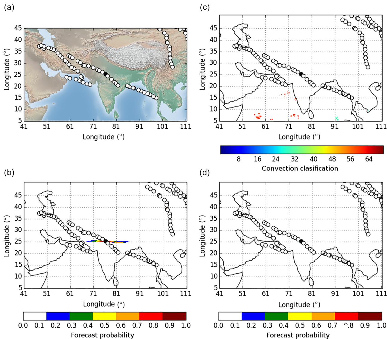
FIGURE 3 Plot of a moderate or greater turbulence event over the possible sources of turbulence: (a) orography, shear turbulence (b) Met Office Global and Regional Ensemble Prediction System [MOGREPS-G] and (d) European Centre for Medium-Range Weather Forecasts Ensemble Prediction System probability forecast) and (c) convection from satellite data. Only the MOGREPS-G ensemble forecasts the shear turbulence event. The circles indicate turbulence observations with white indicating no turbulence, grey indicating light turbulence and black indicating moderate or greater turbulence. The convective classification can be found in Francis and Batstone (2013) [Colour figure can be viewed at wileyonlinelibrary.com ]
