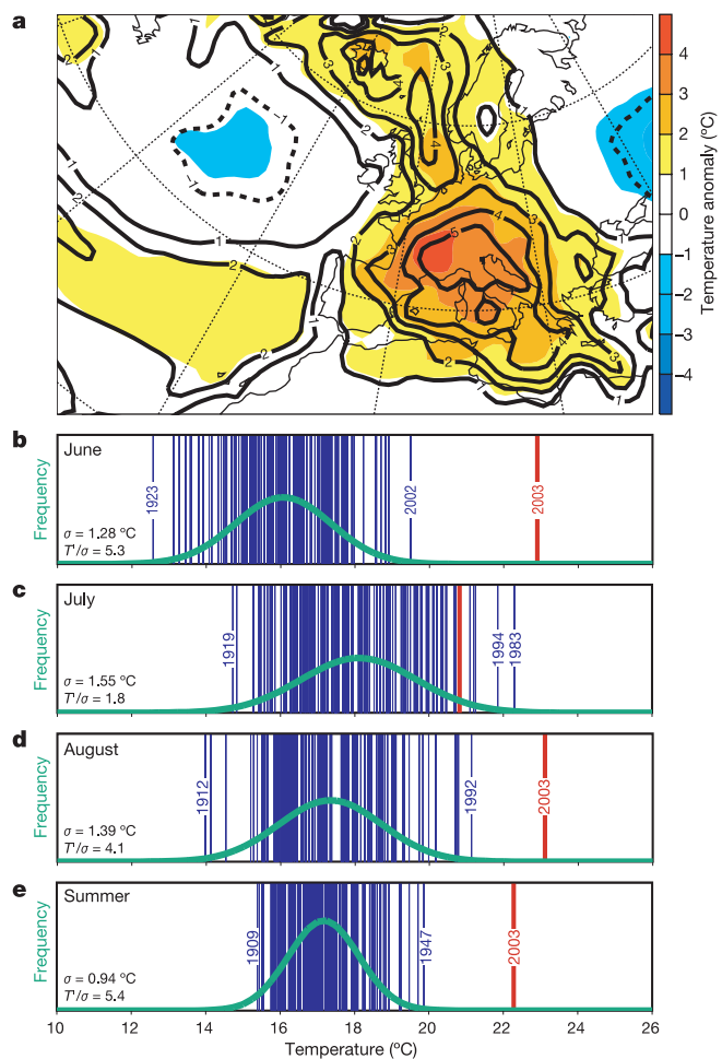
Figure 1 Characteristics of the summer 2003 heatwave. a , JJA temperature anomaly with respect to the 1961–90 mean. Colour shading shows temperature anomaly ( ^\circ\text{C} ), bold contours display anomalies normalized by the 30-yr standard deviation. b–e , Distribution of Swiss monthly and seasonal summer temperatures for 1864–2003. The fitted gaussian distribution is indicated in green. The values in the lower left corner of each panel list the standard deviation ( \sigma ) and the 2003 anomaly normalized by the 1864–2000 standard deviation ( T'/\sigma ). See Methods section for further details.
