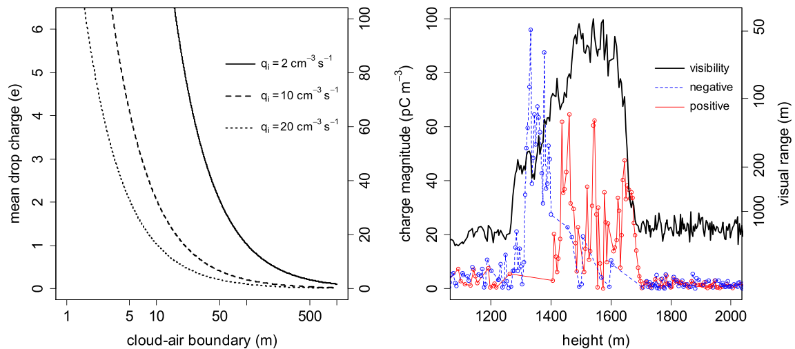
Figure 9. (a) Calculation of mean drop charge with cloud–air boundary thickness for a range of ion production rates q_i and 10\ \mu\text{m} radius drops, with (right-hand axis) the equivalent charge density for N_d = 100\ \text{drops cm}^{-3} . Assumptions: conduction current density J_c = 2\ \text{pA m}^{-2} , air temperature 273\ \text{K} . (b) Positive (red line) and negative (blue line) charge density plotted with height, with the visual range determination (black line) also shown (right-hand axis).
