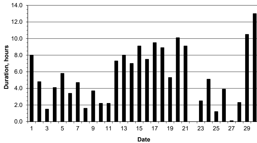
Daily sunshine
