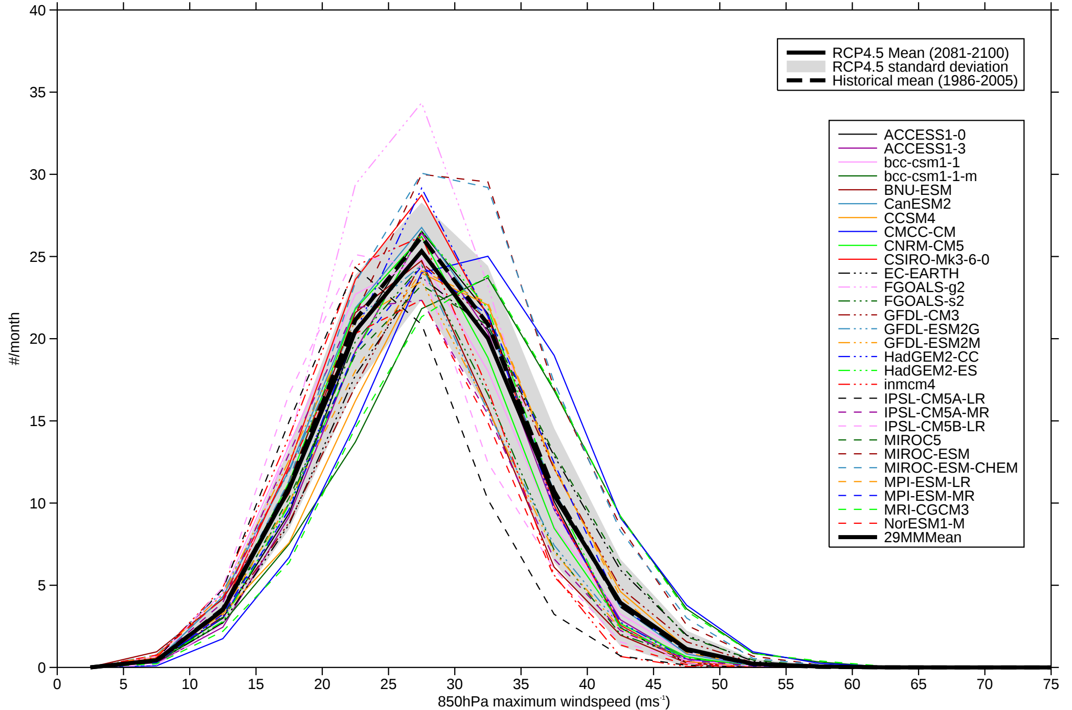
Intensity distribution of 850hPa winds - SH DJF
