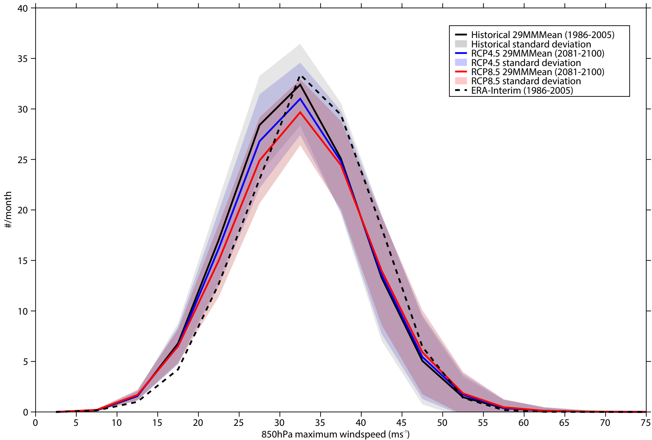
Intensity distribution of 850hPa Winds - SH JJA
