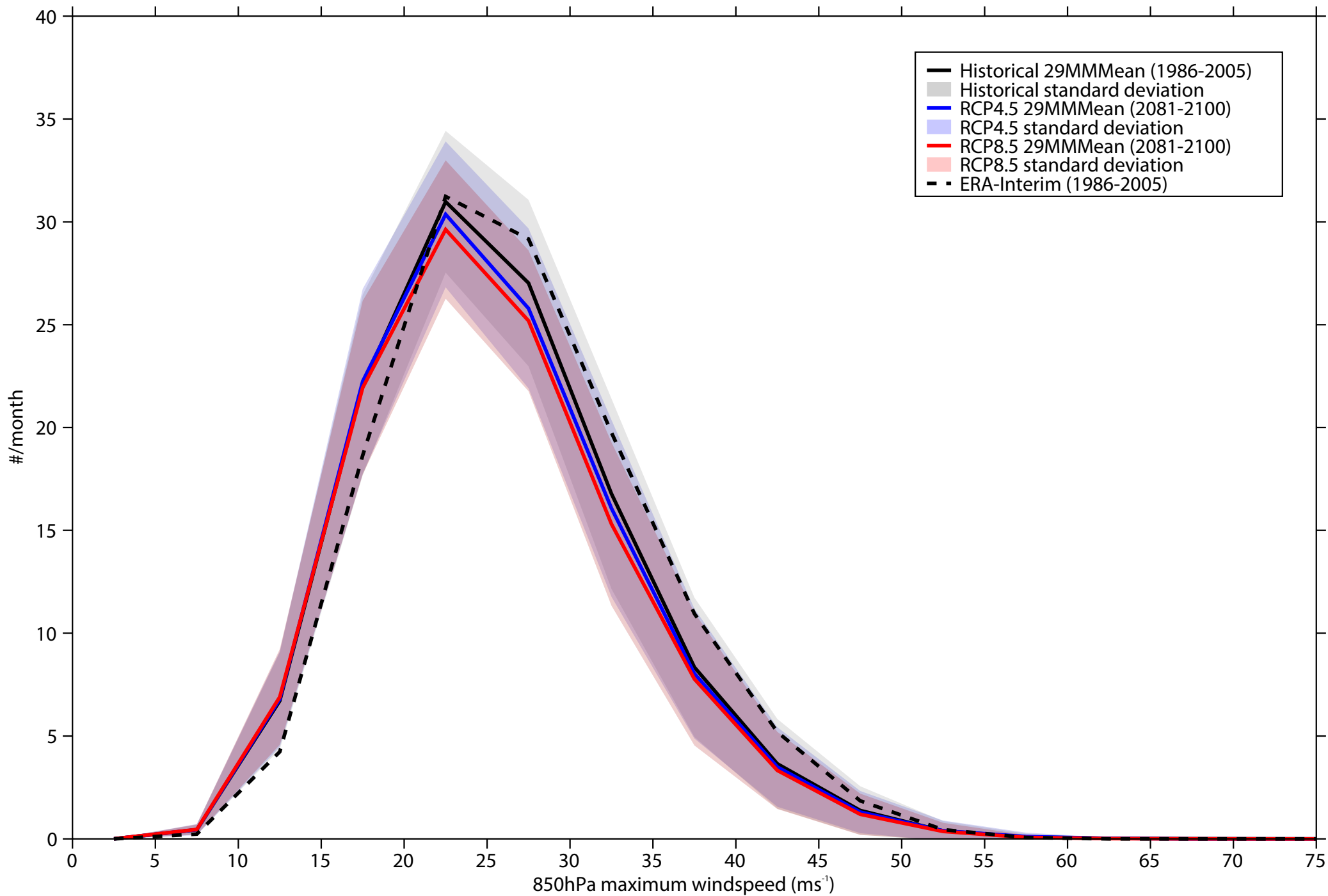
Intensity distribution of 850hPa Winds - NH MAM
