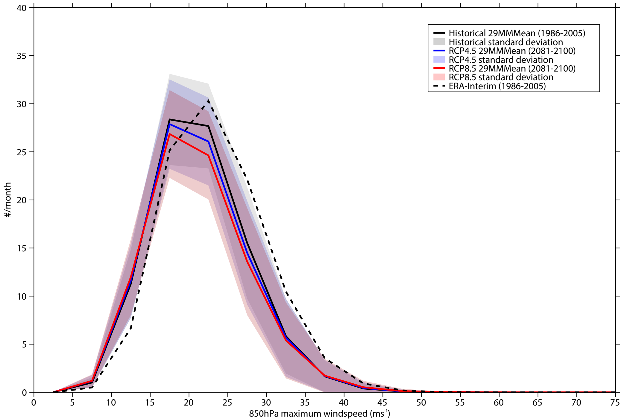
Intensity distribution of 850hPa Winds - NH JJA
