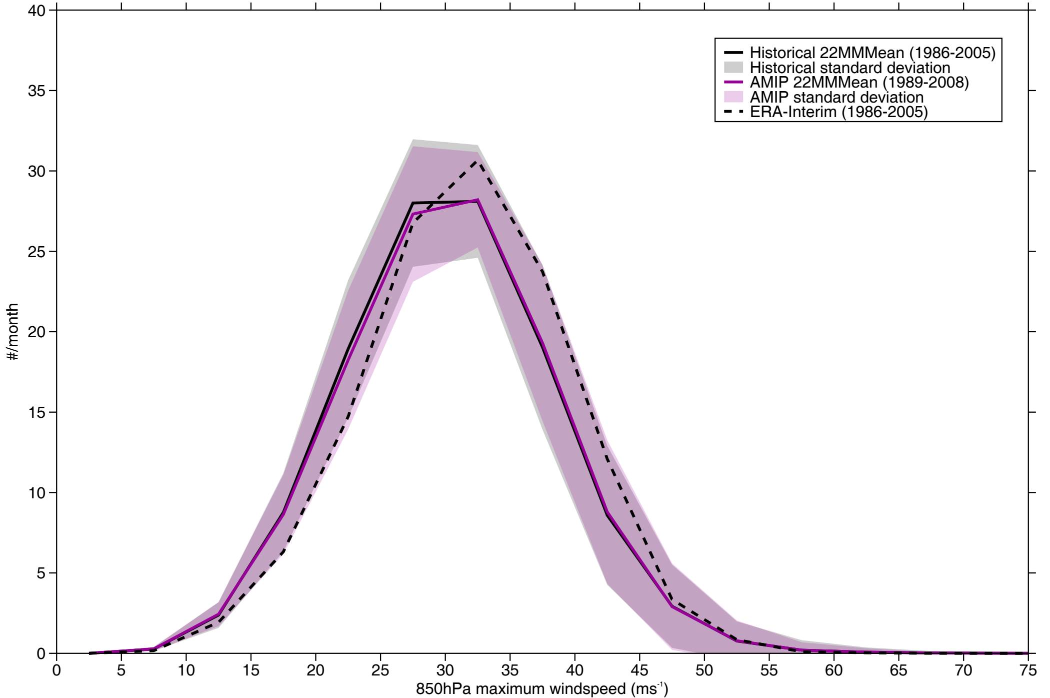
Intensity distribution of 850hPa Winds - SH SON
