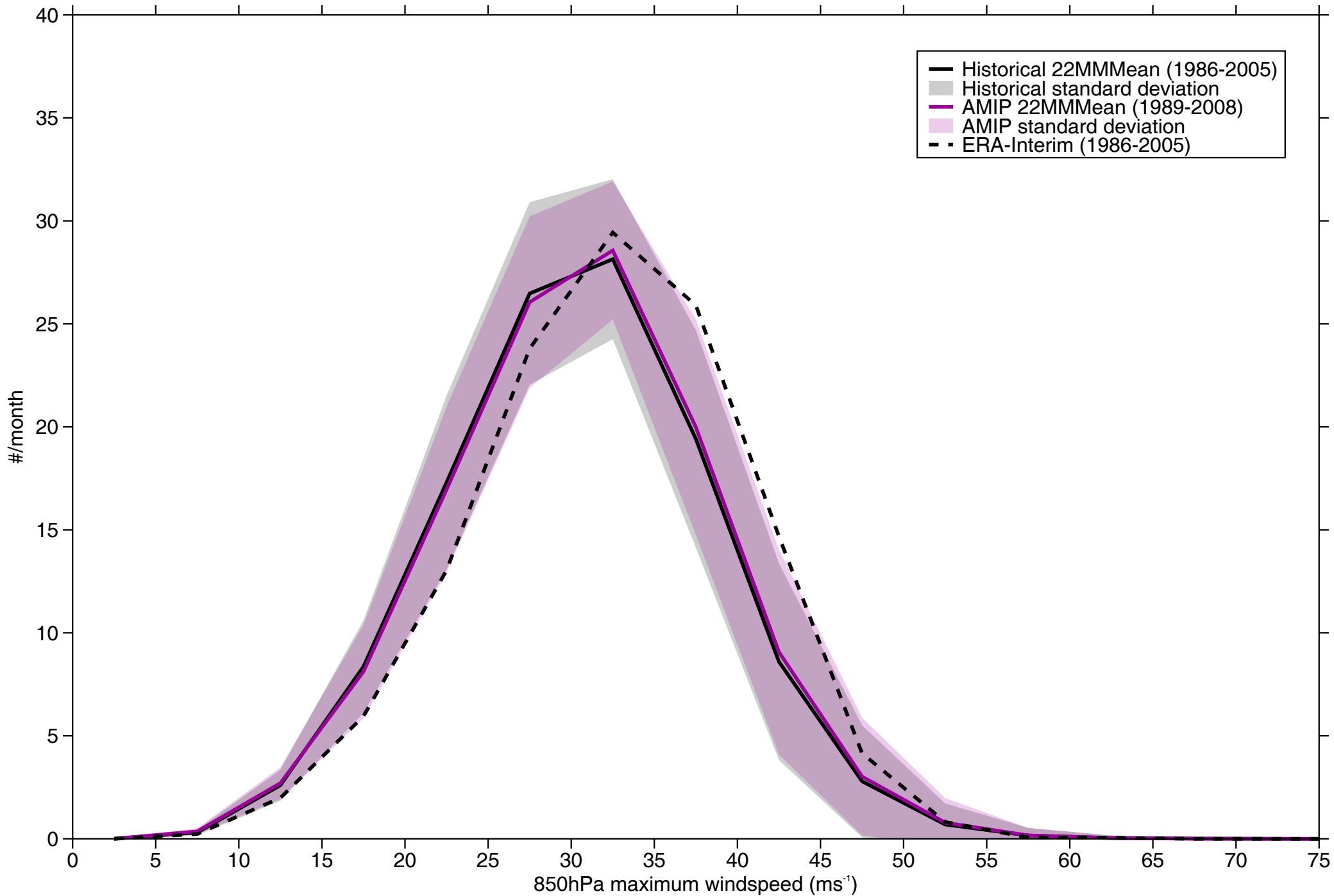
Intensity distribution of 850hPa Winds - SH MAM
