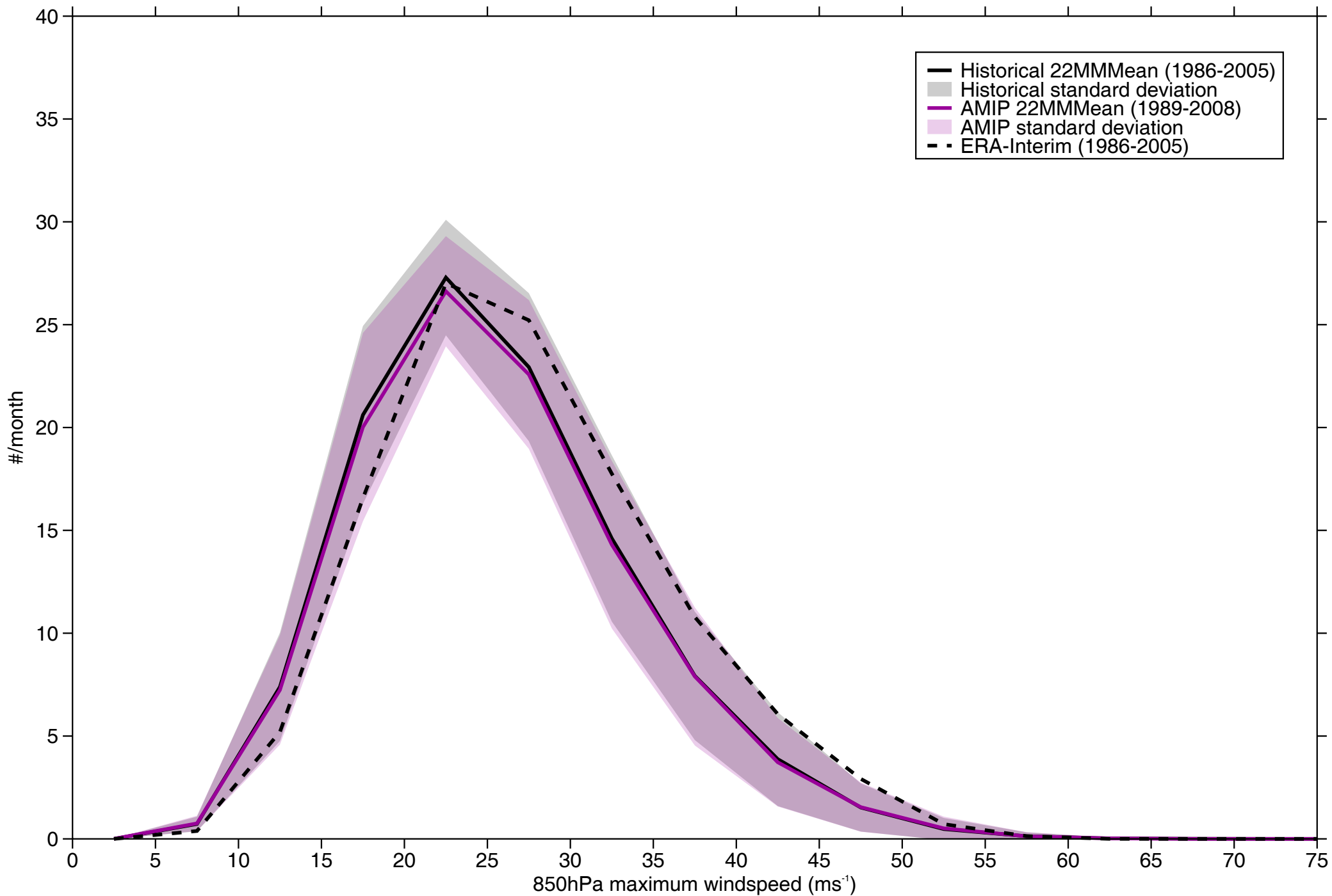
Intensity distribution of 850hPa Winds - NH SON
