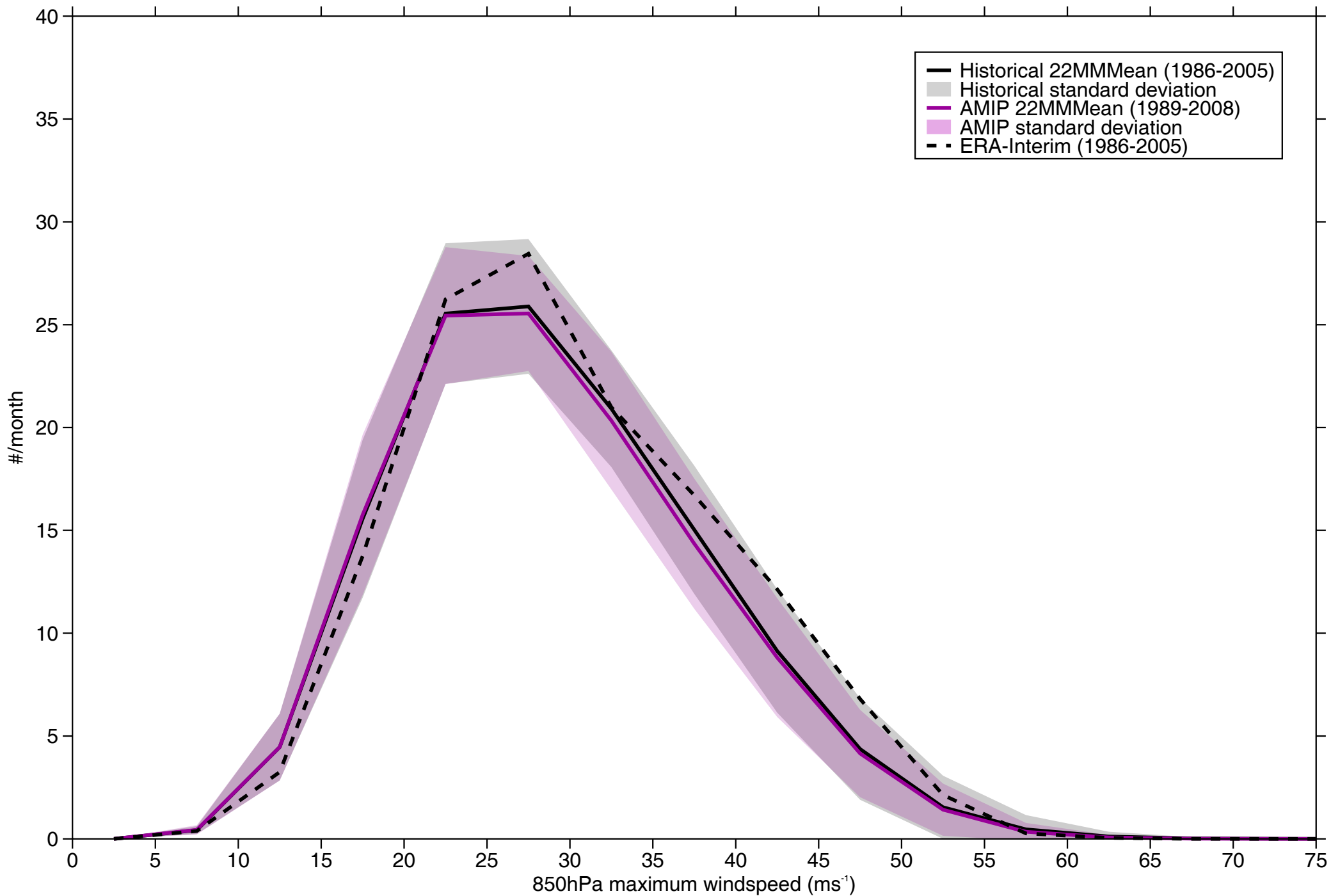
Intensity distribution of 850hPa Winds - NH DJF
