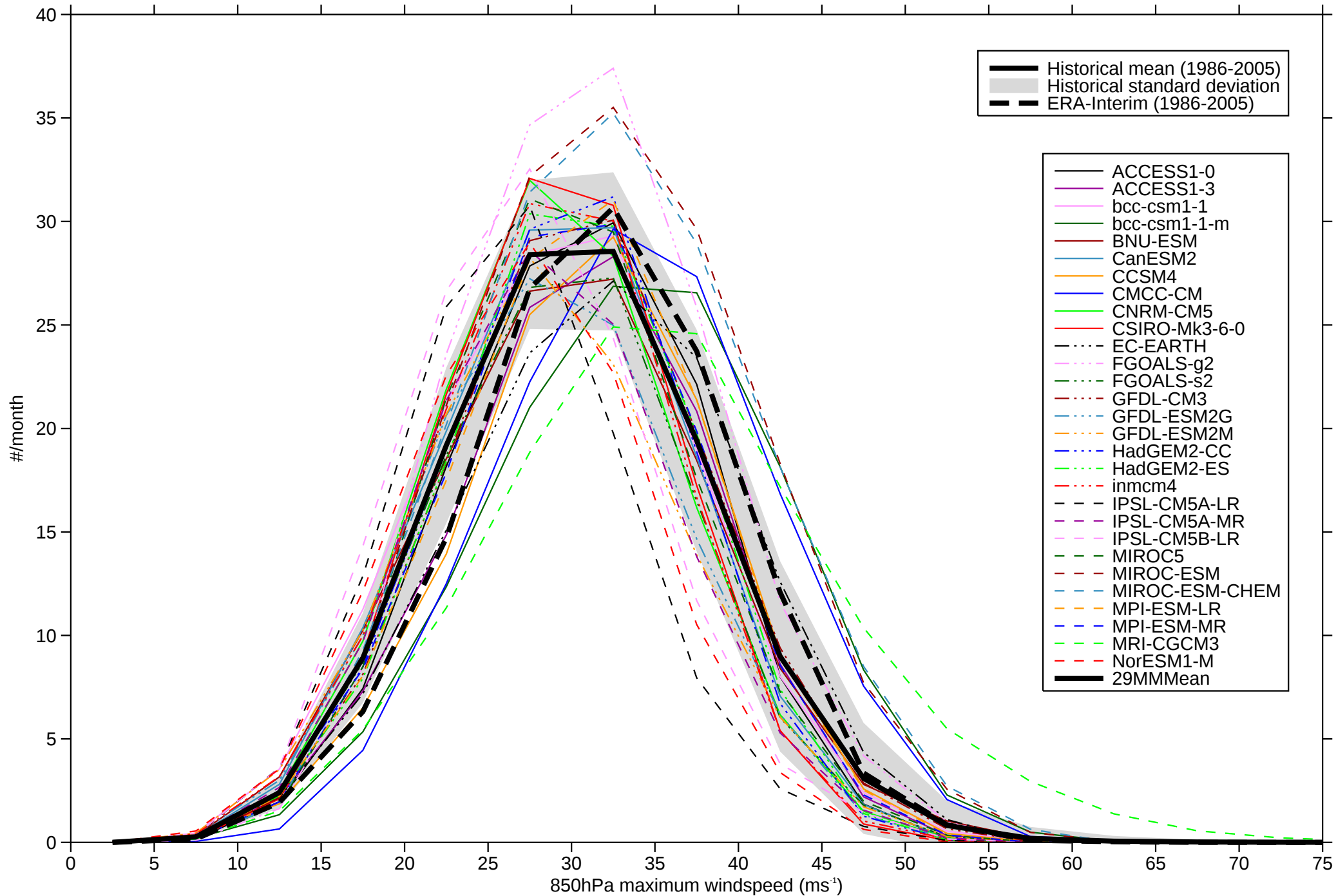
Intensity distribution of 850hPa winds - SH SON
