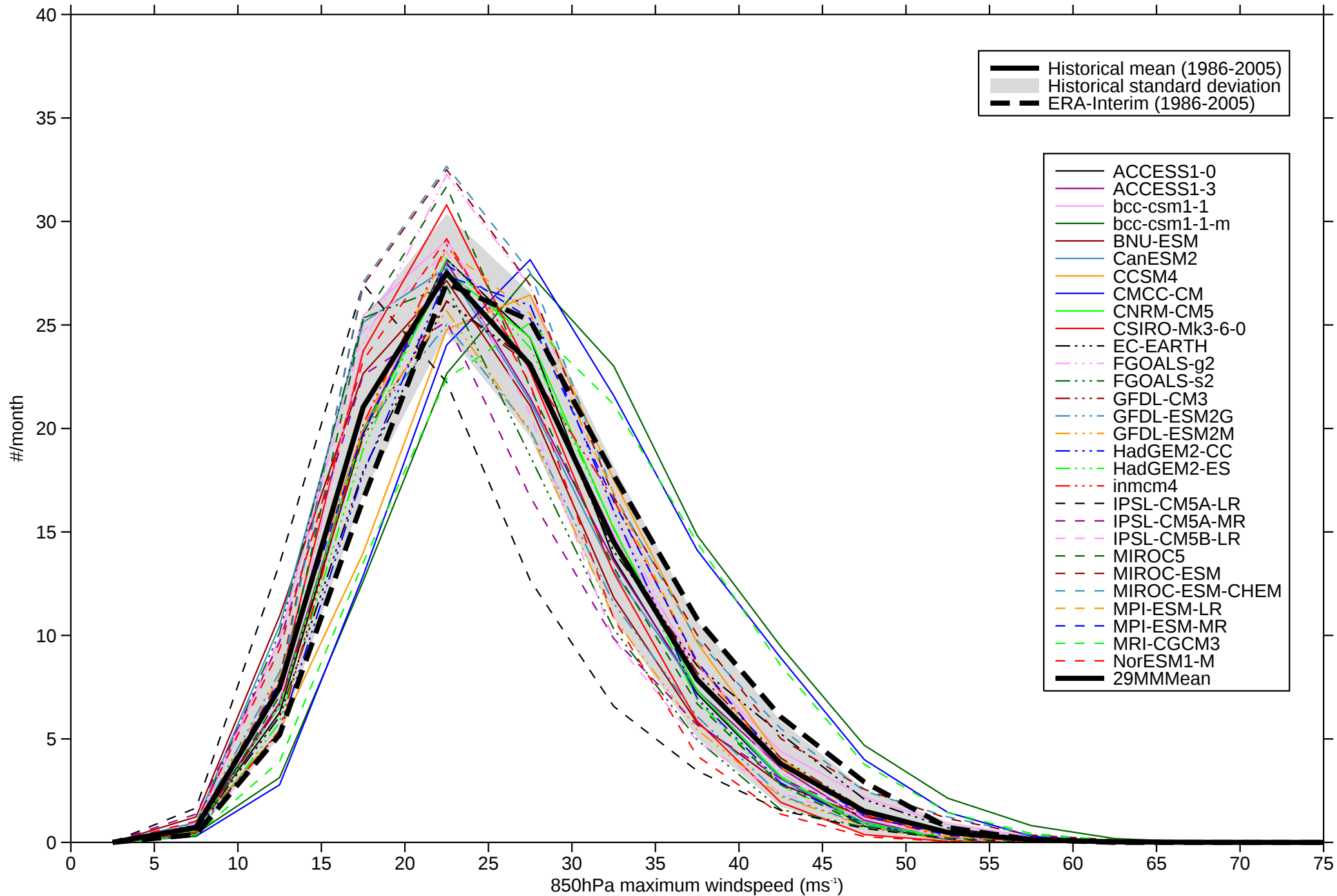
Intensity distribution of 850hPa winds - NH SON
