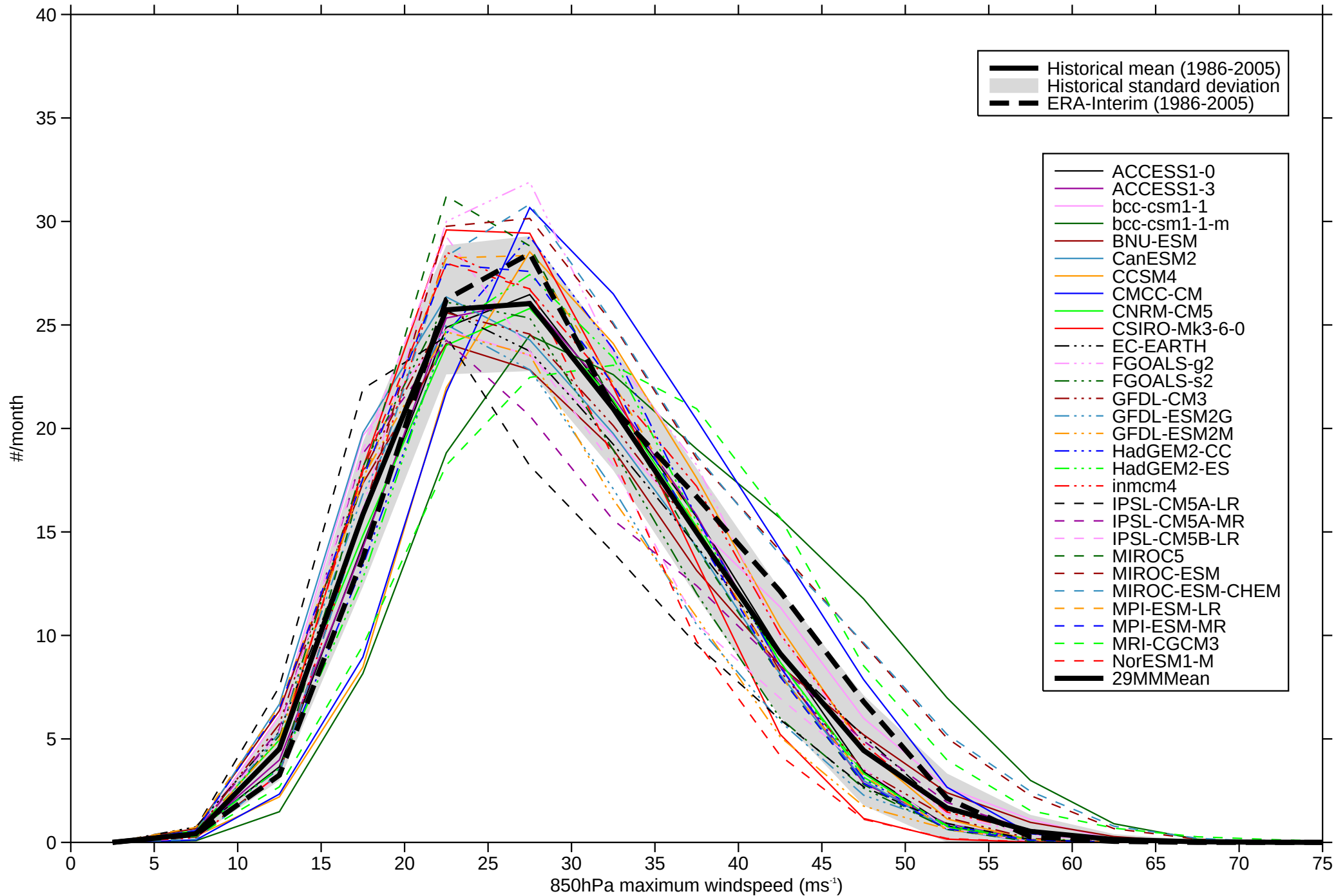
Intensity distribution of 850hPa winds - NH DJF
