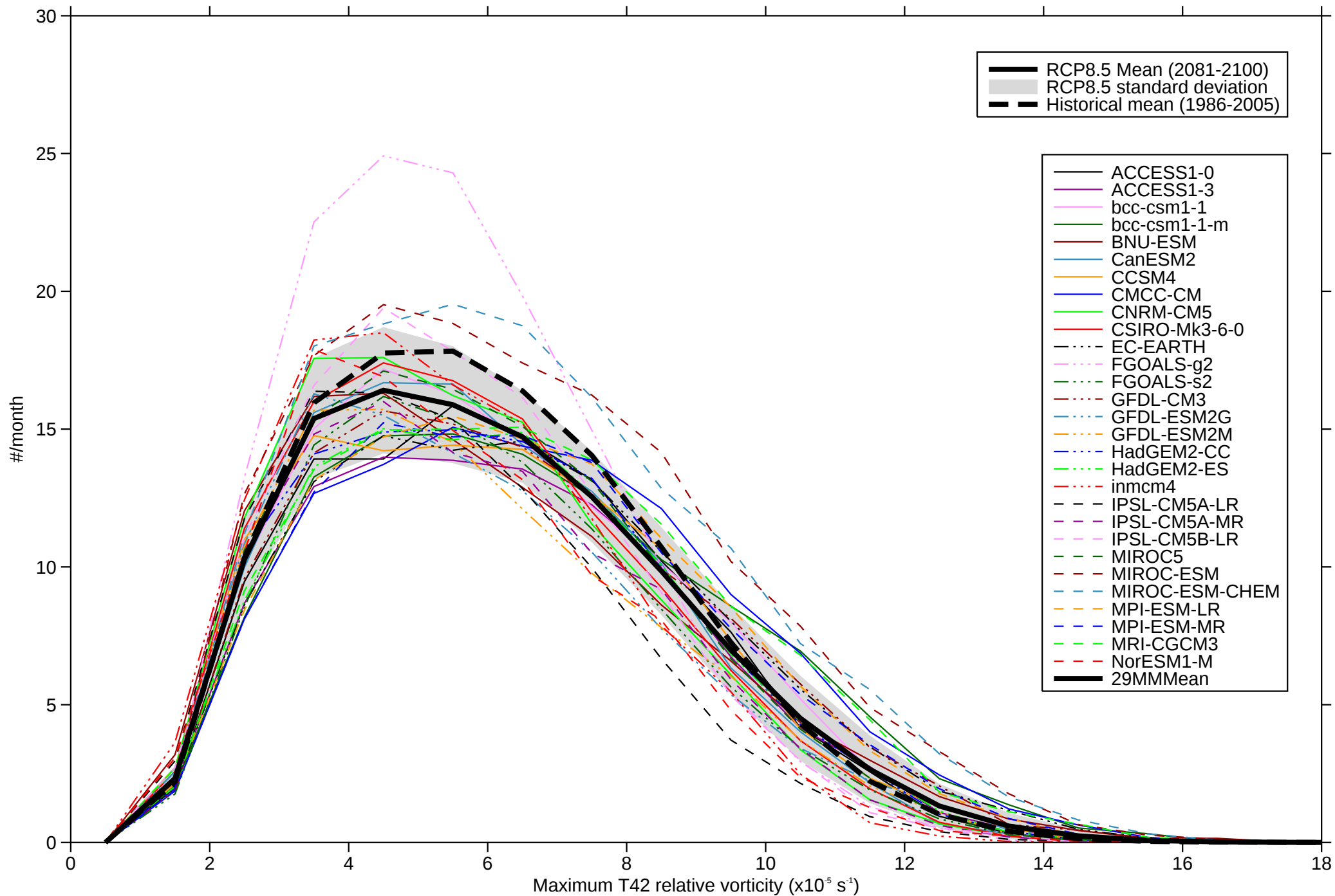
Intensity distribution of maximum T42 relative vorticity - SH SON
