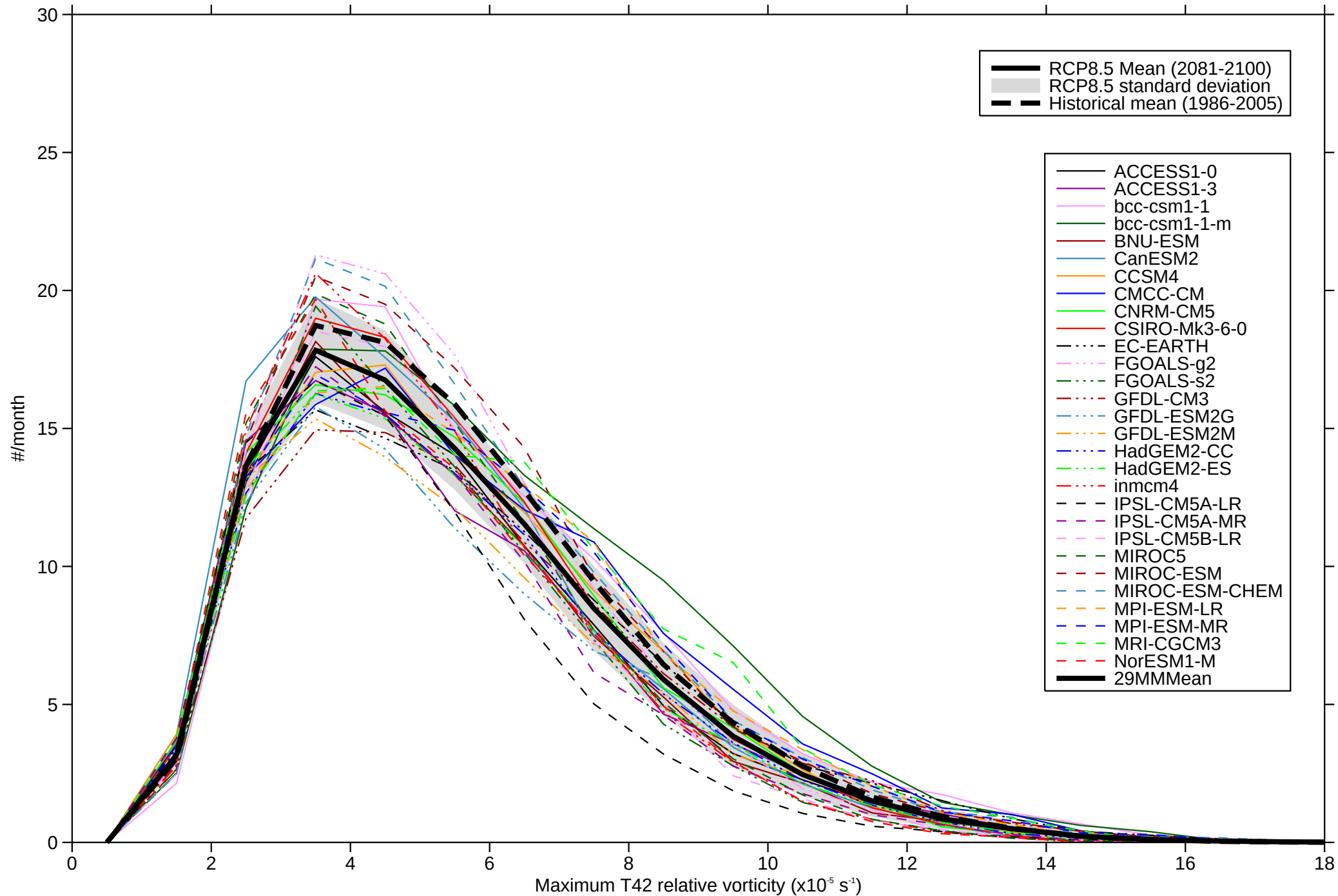
Intensity distribution of maximum T42 relative vorticity - NH SON
