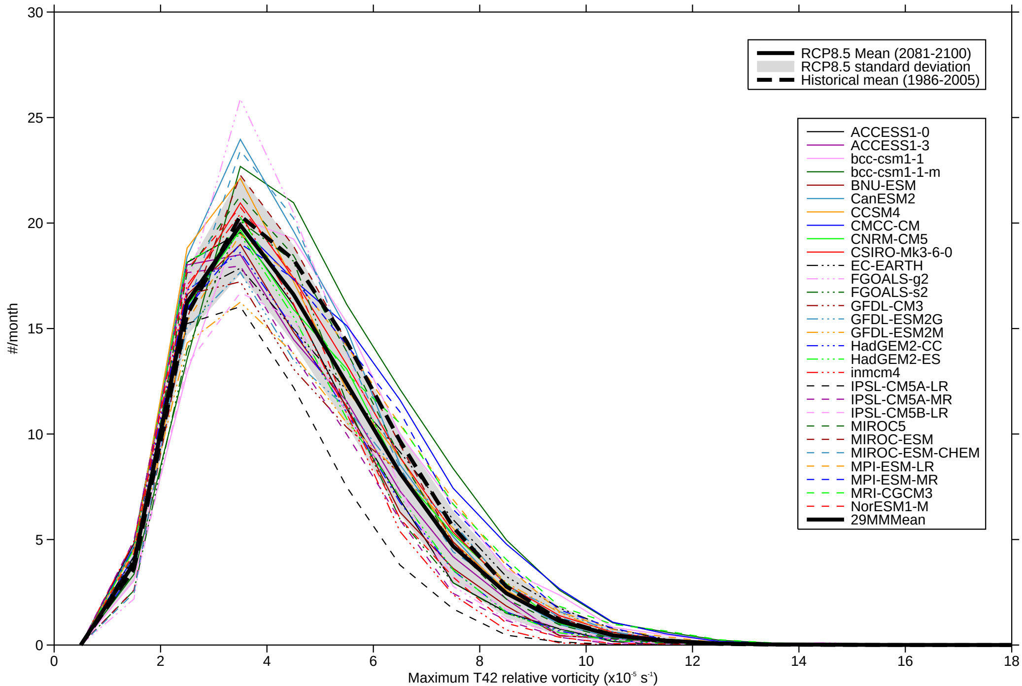
Intensity distribution of maximum T42 relative vorticity - NH JJA
