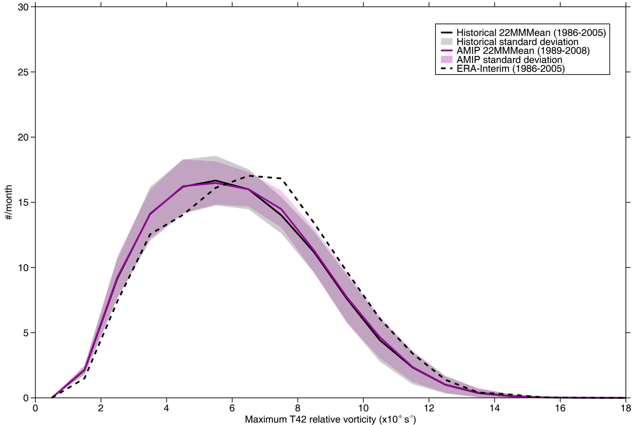
Intensity distribution of maximum T42 relative vorticity - SH MAM
