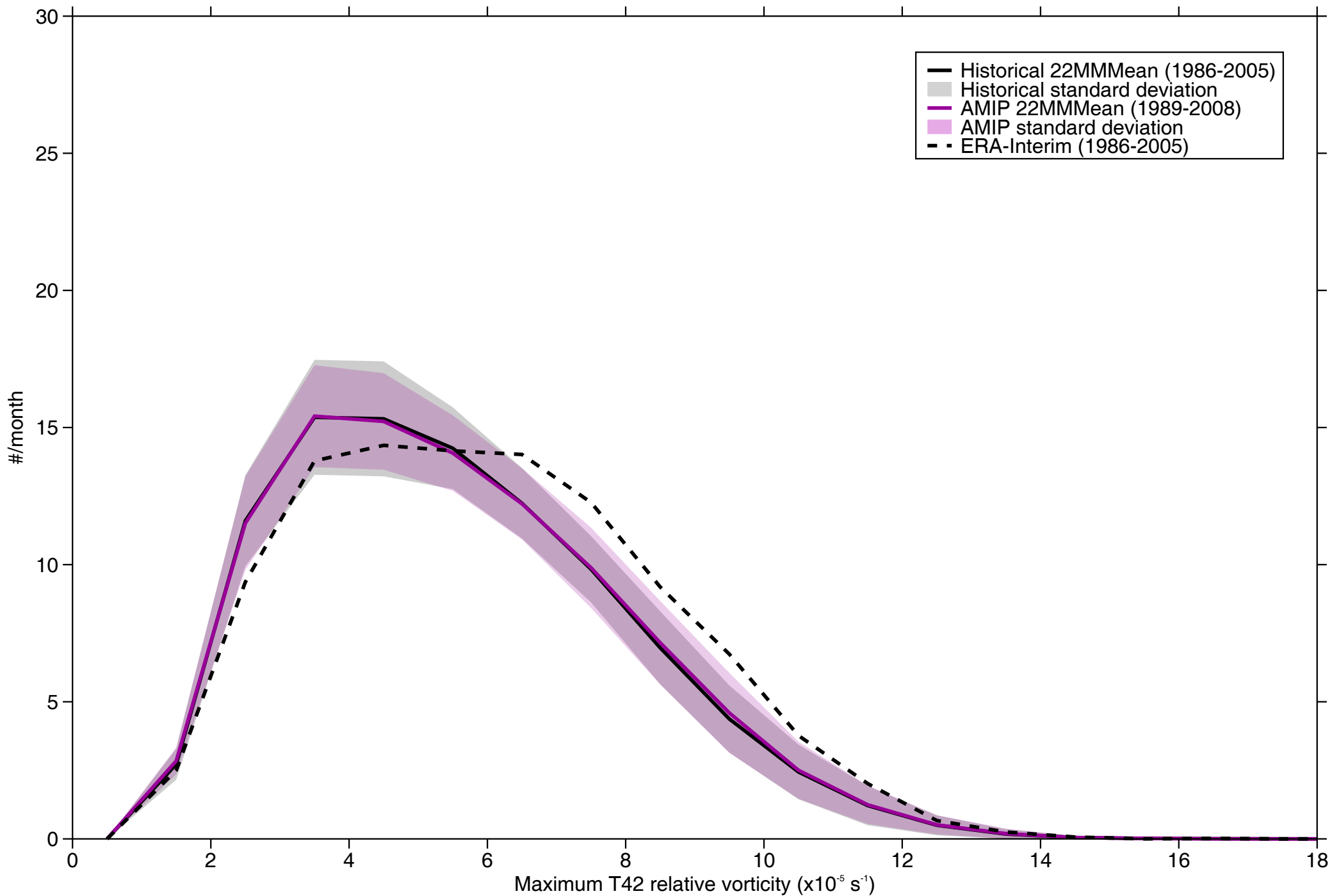
Intensity distribution of maximum T42 relative vorticity - SH DJF
