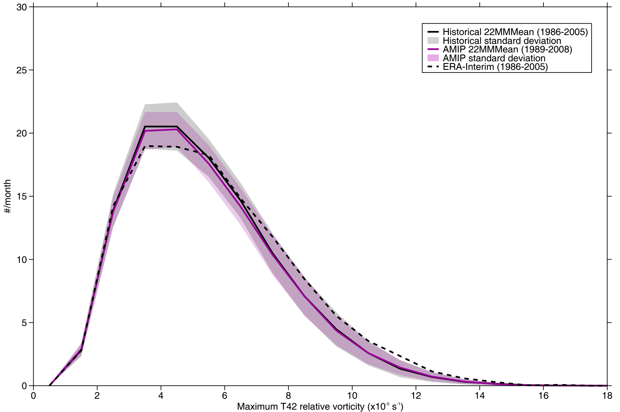
Intensity distribution of maximum T42 relative vorticity - NH MAM
