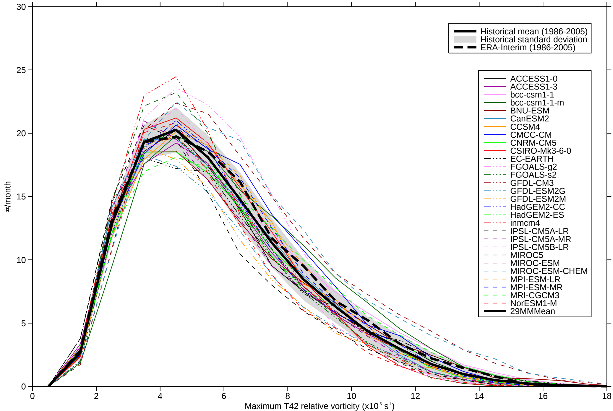
Intensity distribution of maximum T42 relative vorticity - NH DJF
