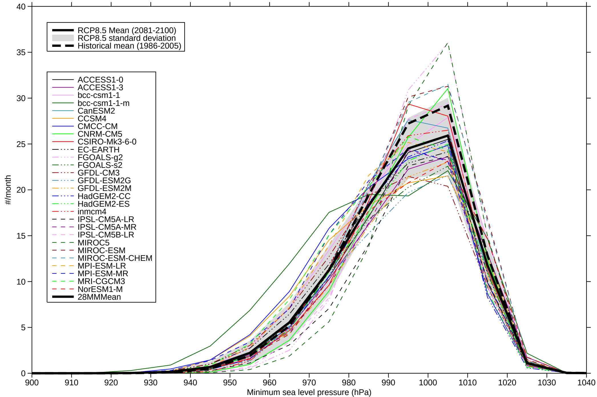
Intensity distribution of minimum sea level pressure - NH SON
