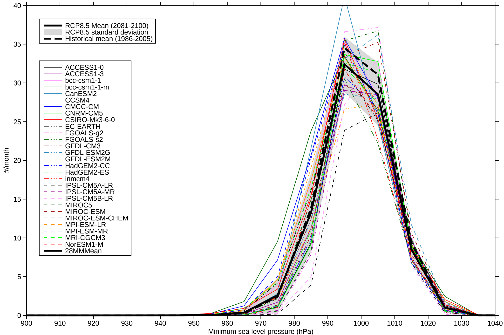
Intensity distribution of minimum sea level pressure - NH JJA
