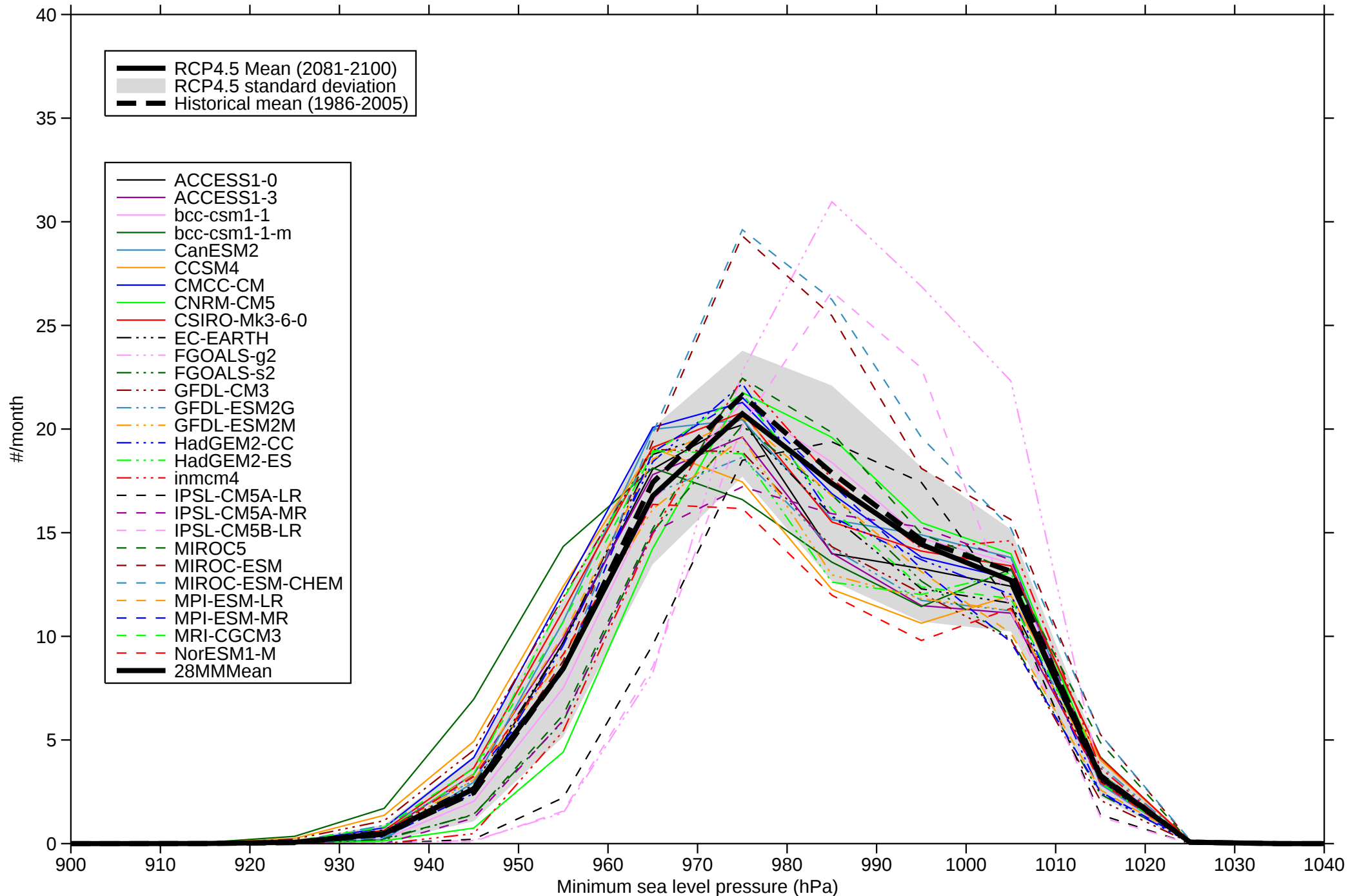
Intensity distribution of minimum sea level pressure - SH DJF
