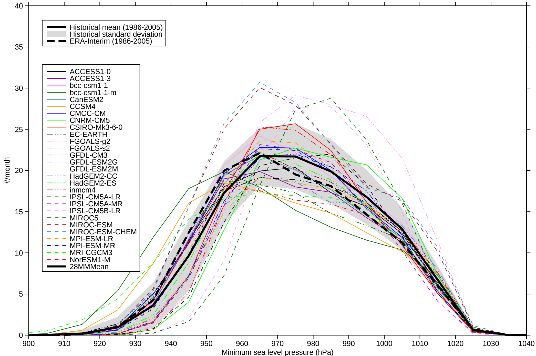
Intensity distribution of minimum sea level pressure - SH JJA
