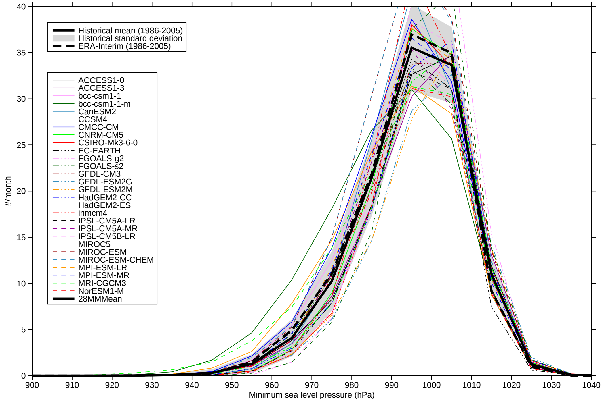
Intensity distribution of minimum sea level pressure - NH MAM
