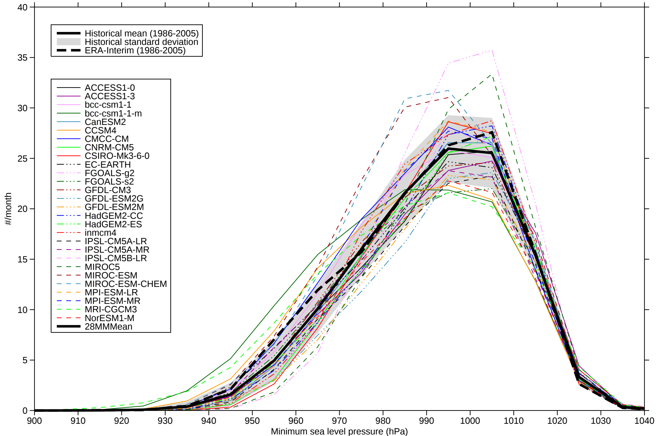
Intensity distribution of minimum sea level pressure - NH DJF
