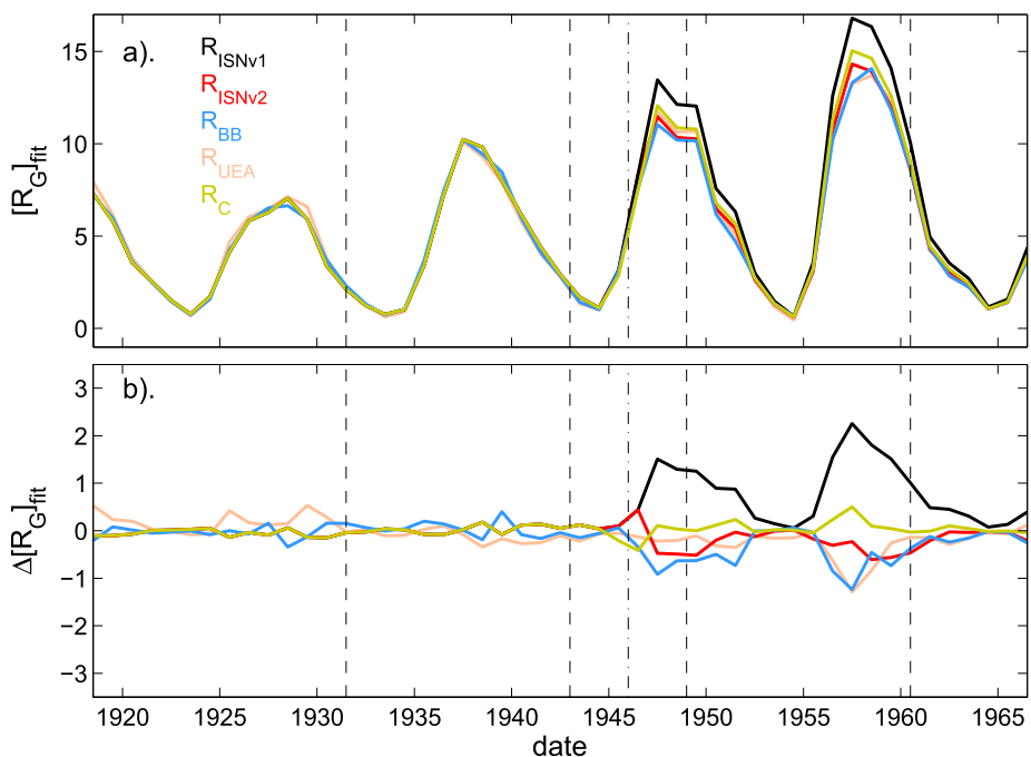
Figure 1 Comparison of the tested sunspot data series: (black) R_{\text{ISNV1}} , (red) R_{\text{ISNV2}} , (blue) R_{\text{BB}} , (pink) R_{\text{UEA}} , and (olive) R_C . To enable easy comparison, all have been scaled by linear regression to the RGO sunspot-group number [ N_G ] over the interval 1921 – 1945. The top panel shows the regressed time series, and the bottom panel shows the differences between each regressed variation and the average of the five scaled tested series. The vertical dot-dashed line is the most likely time of the Waldmeier discontinuity (1946), and the vertical-dashed lines delineate the optimum “before” and “after” intervals found by the analysis.
