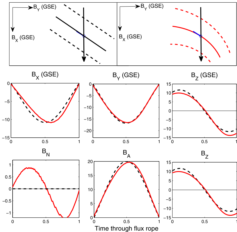
Figure 3 Top panels: Axes (solid lines) and boundaries (dashed lines) of straight-axis force-free (black) and curved (red) flux ropes in the X-Y (GSE) plane. The large black arrows represent spacecraft trajectories through the structures, which have the same local axis orientation at the point of spacecraft intercept. Middle panels: Magnetic field vectors in GSE coordinates as simulated along the spacecraft trajectory in function of a normalised coordinate (0: entrance, 1: exit). Bottom panels: Magnetic field vectors in the flux rope coordinate system.
