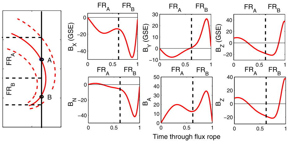
Figure 5 An example of an encounter with a curved flux rope which results in a magnetic field time series which could be interpreted (and modelled) as a ‘double flux rope’. The three top right panels are in GSE coordinates, while the three bottom right panels are in flux rope coordinates at A. Choosing the boundary between the two axis encounters, FR_A and FR_B , is somewhat subjective.
