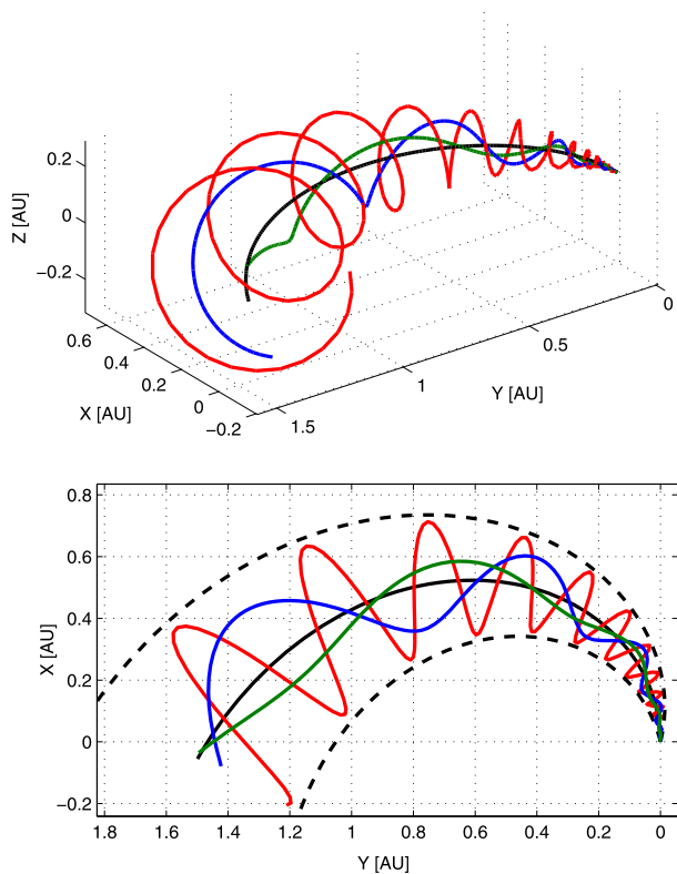
Figure 1 The curved magnetic flux rope model used in this study. While we do not expect magnetic clouds (MCs) to have this global configuration, particularly to have axes aligned with the Parker spiral, it is a useful construct to investigate local morphology. The top panel shows the three-dimensional structure, with black, green, blue and red showing magnetic field lines at a normalised distance from the axis of r = 0, 0.3, 0.6 and 0.9 , respectively. The bottom panel shows the projection onto the solar rotation ( i.e. , R-\theta ) plane. The black dashed lines indicate the front and rear boundaries of the flux rope, as defined by r = 1 .
