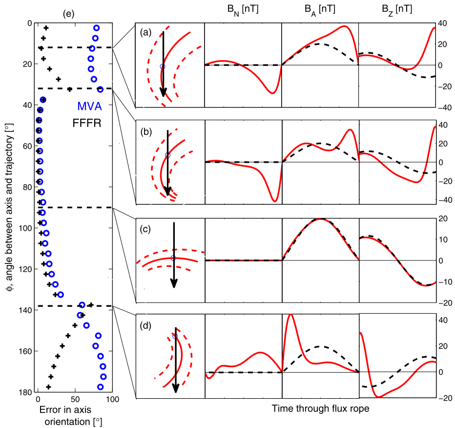
Figure 4 Effect of \phi , the angle between the spacecraft trajectory and axis, on MC reconstruction. The black arrows in panels a–d show four different spacecraft trajectories through the curved flux rope. Next to each trajectory is the curved (red) and force-free (black dashed) flux rope time series (in the local flux rope coordinate system defined by the model with A along the flux rope axis and N normal to it). Panel e shows the error in the axis estimation from MVA (black) and FFFR fitting (blue) with \phi .
