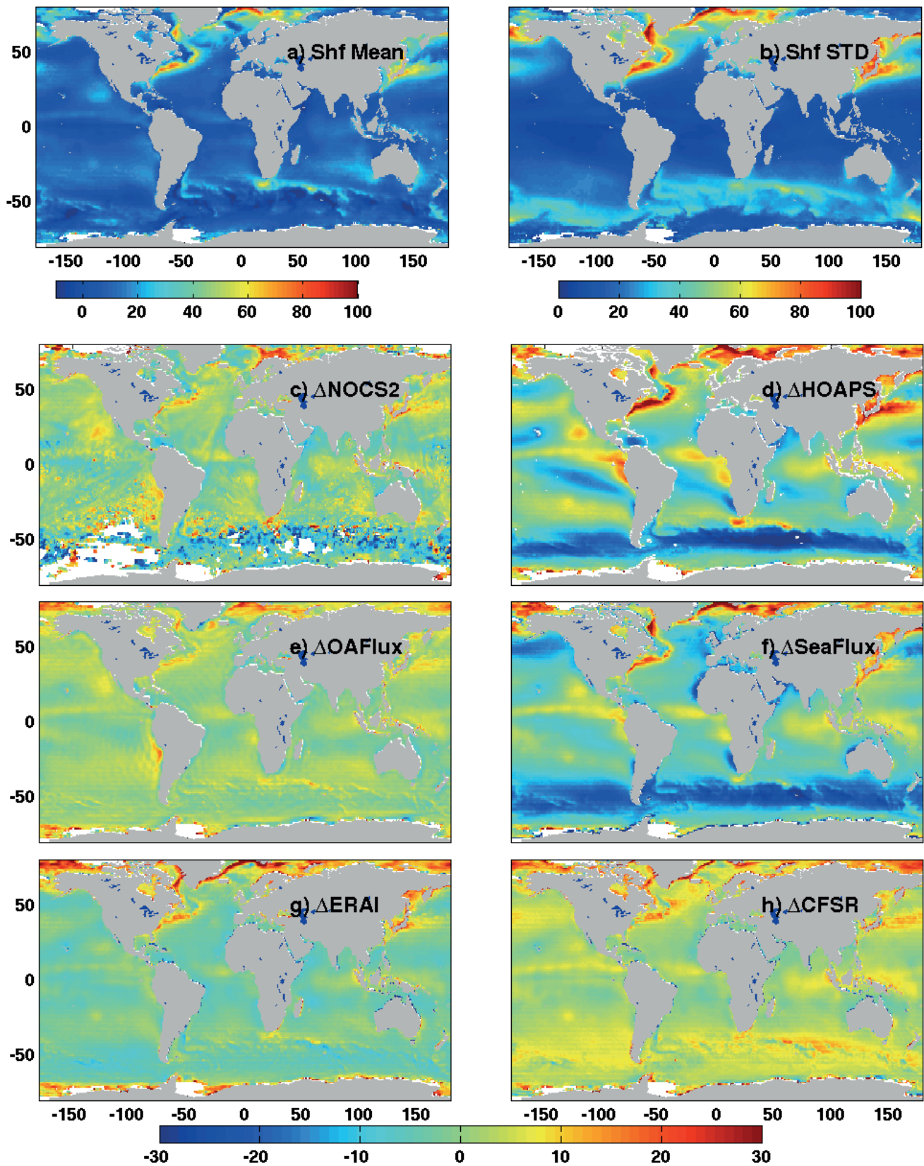
Fig. 2: Annual mean (a) of IFREMER SHF (2000 - 2007) and of the associated variability (STD) (b). Mean differences of SHF derived from IFREMER and from c) NOCS2, d) HOAPS, e) OAFflux, f) SeaFlux, g) ERA Interim, and h) CFRS. Units are W/m^2 .
