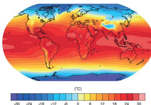
Fig.1: Multi-model (ensemble) annual mean surface (2 m) air temperature ( ^{\circ}\text{C} ) for the period 1980-2005 constructed with one realization of all available models used in the CMIP5 historical experiment. Adopted from Flato et al. 2013.
