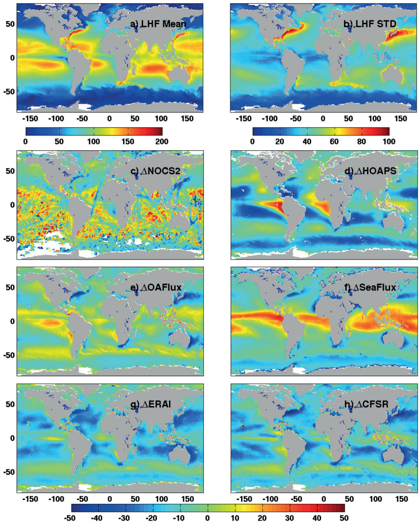
Fig. 1: Annual mean (a) of IFREMER LHF (2000 - 2007) and of the associated variability (STD) (b). Mean differences of LHF derived from IFREMER and from c) NOCS2, d) HOARS, e) OAFux, f) SeaFlux, g) ERA Interim, and h) CFRS. Units are W/m².
