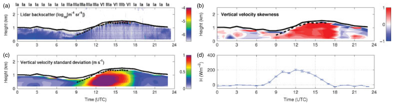
Figure 3. Observations taken on 11 September 2009: (a) attenuated lidar backscatter coefficient with the most probable boundary-layer type shown in Roman numerals, (b) 2-hourly mean skewness of vertical velocity, (c) 2-hourly mean standard deviation of vertical velocity, (d) hourly-mean surface sensible heat flux. In (a), (b) and (c) the solid black indicates the diagnosed boundary-layer top and the dashed line indicates the diagnosed cloud base.
