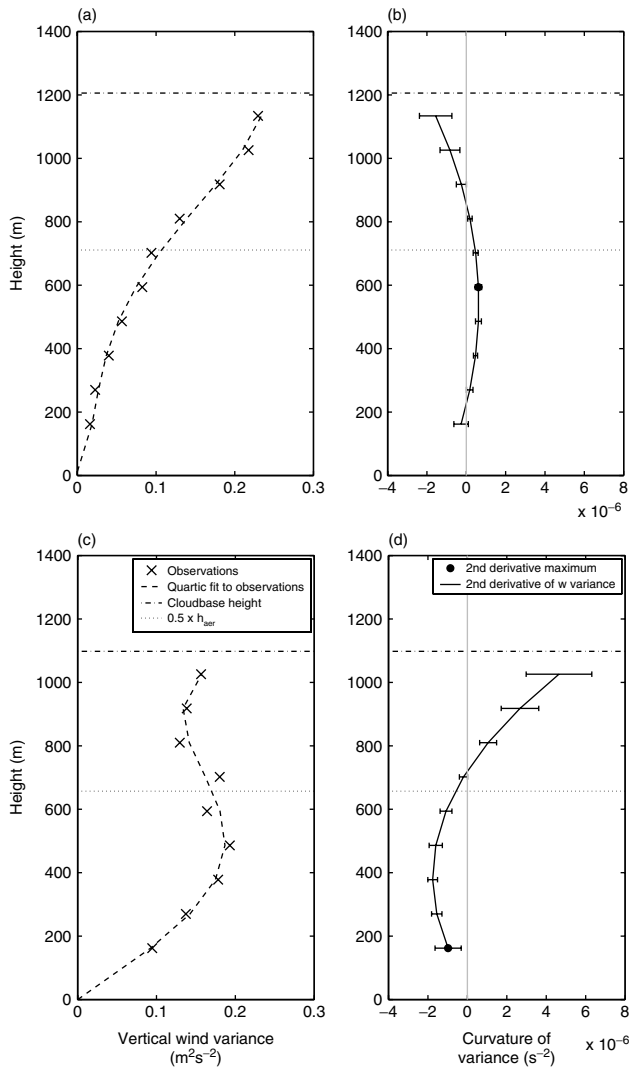
Figure 6. (a) Vertical profile of 2-hourly mean vertical velocity variance observations (crosses) and its corresponding quartic fit (dashed line) for a decoupled boundary layer at 0900 UTC on 18 October 2009. Also shown are the cloud base height (dot-dash line) and the height of the lower half of the boundary layer (dotted line). (b) Vertical profile of the second derivative of the fit of vertical velocity variance and associated error (solid black line). The black circle denotes the height of the maximum curvature of vertical velocity variance in the lower half of the boundary layer, which the algorithm uses to assess the probability of the boundary layer being decoupled. Panels (c, d) are as (a, b), but for a coupled boundary layer at 1500 UTC on 18 October 2009.
