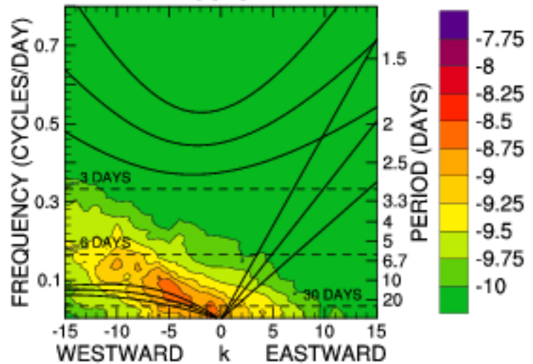
FLAT SYMMETRIC GSFC
