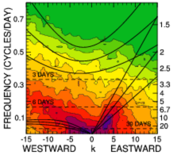
QOBS SYMMETRIC DWD
