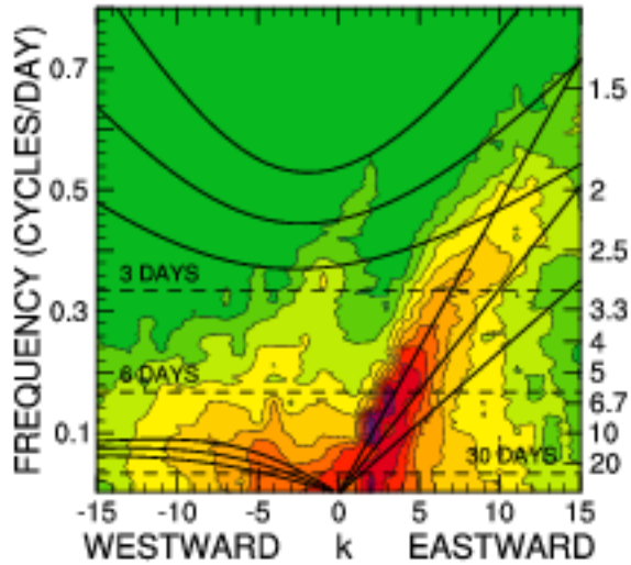
PEAKED SYMMETRIC UKMO.N48
