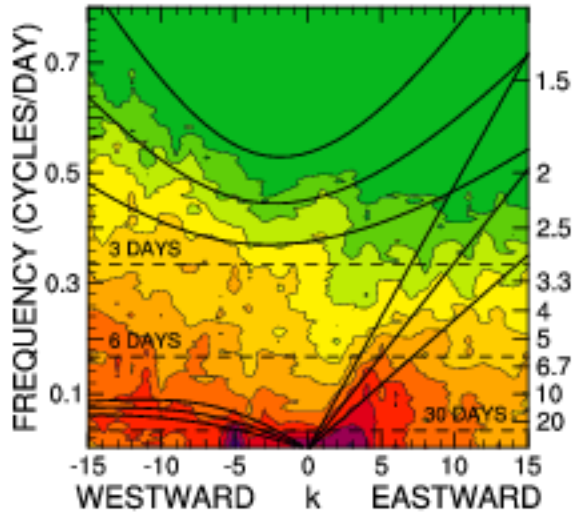
PEAKED SYMMETRIC AGU
