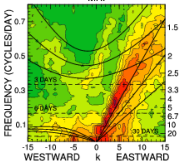
PEAKED SYMMETRIC MRI
