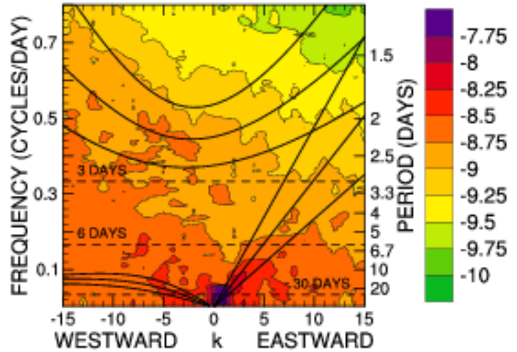
FLAT SYMMETRIC LASG
