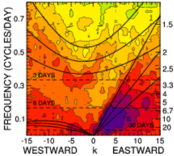
PEAKED SYMMETRIC LASG
