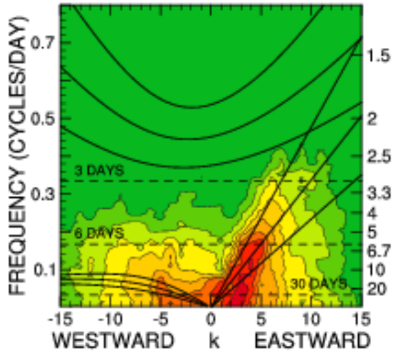
PEAKED SYMMETRIC CGAM
