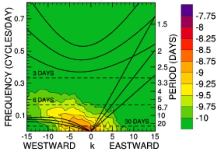
FLAT SYMMETRIC CSIRO
