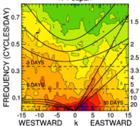
QOBS SYMMETRIC K-1 Japan
