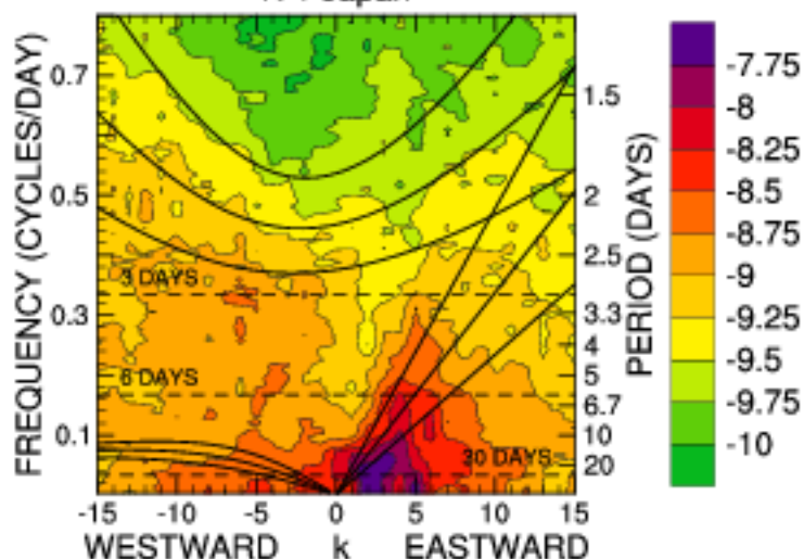
CONTROL SYMMETRIC K-1 Japan
