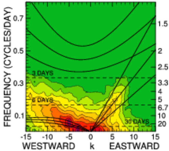
QOBS SYMMETRIC CGAM
