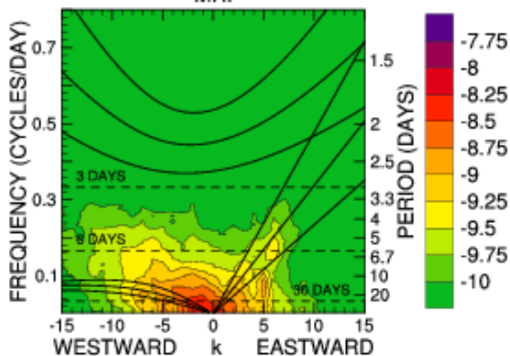
FLAT SYMMETRIC MRI
