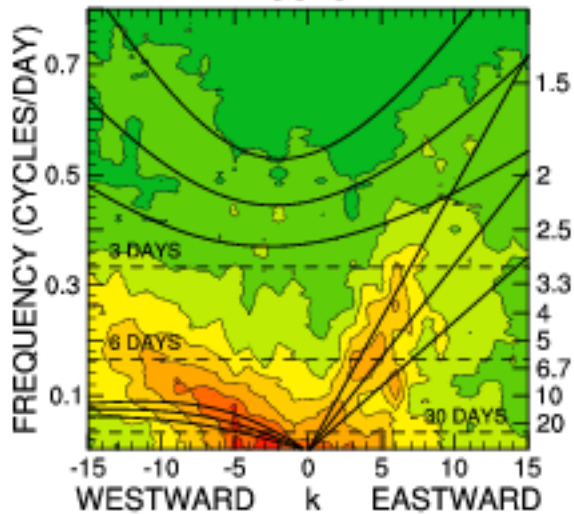
QOBS SYMMETRIC GSFC
