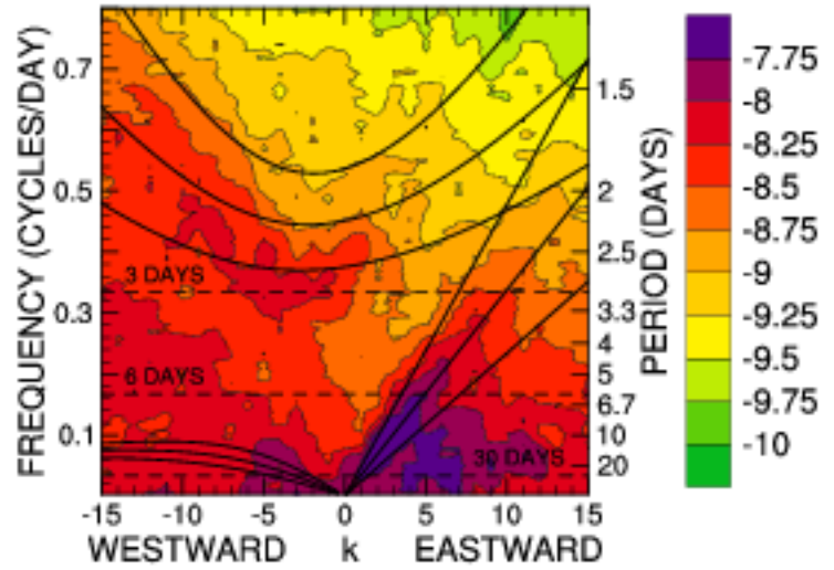
CONTROL SYMMETRIC LASG
