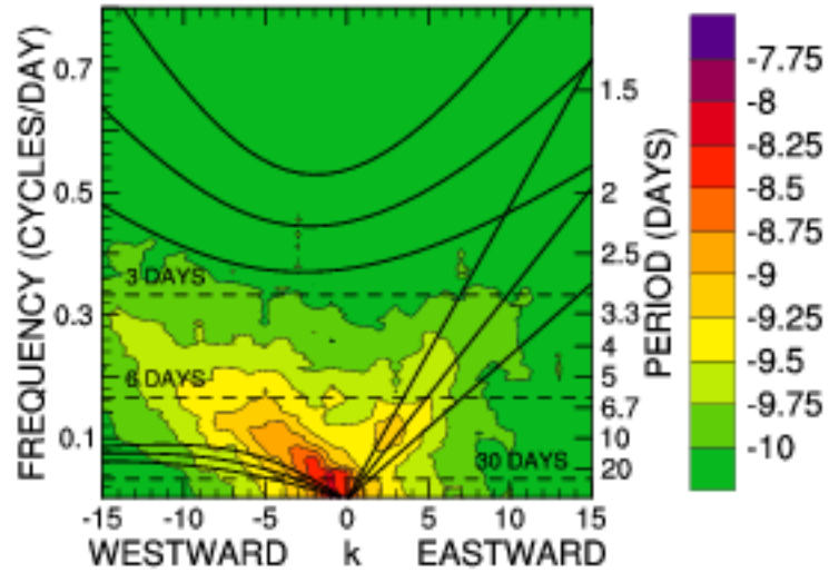
FLAT SYMMETRIC NCAR
