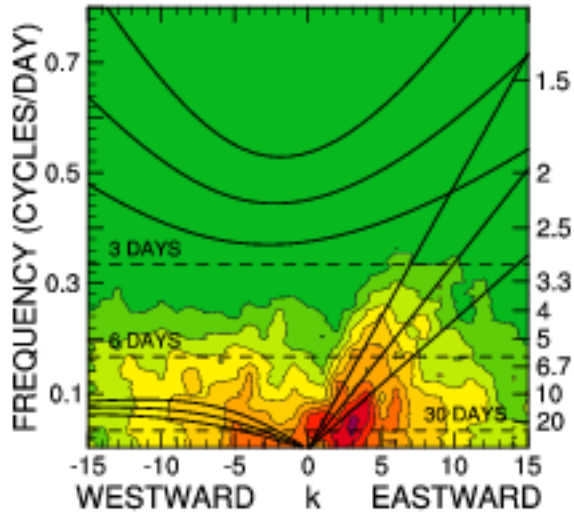
PEAKED SYMMETRIC CSIRO
