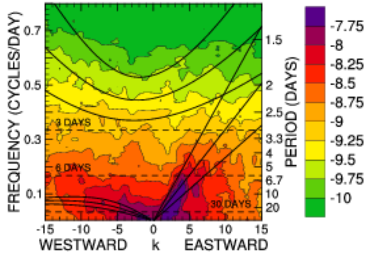
CONTROL SYMMETRIC DWD
