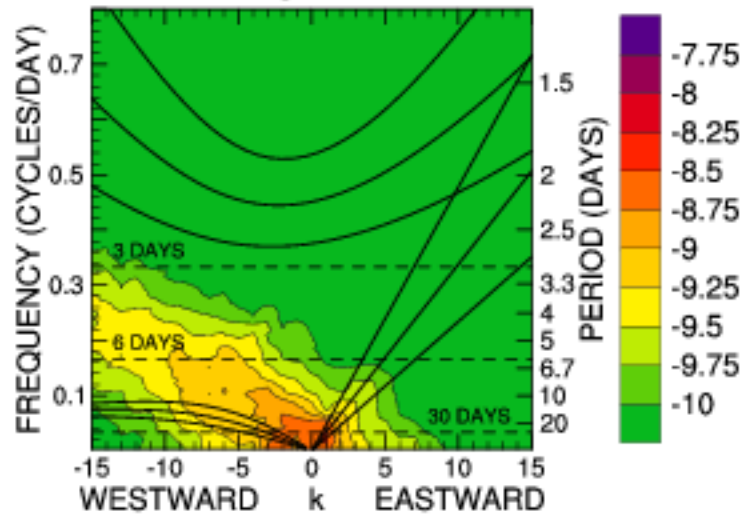
FLAT SYMMETRIC ECMWF
