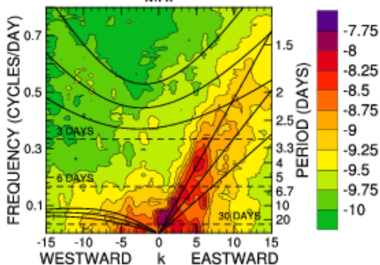
CONTROL SYMMETRIC MRI
