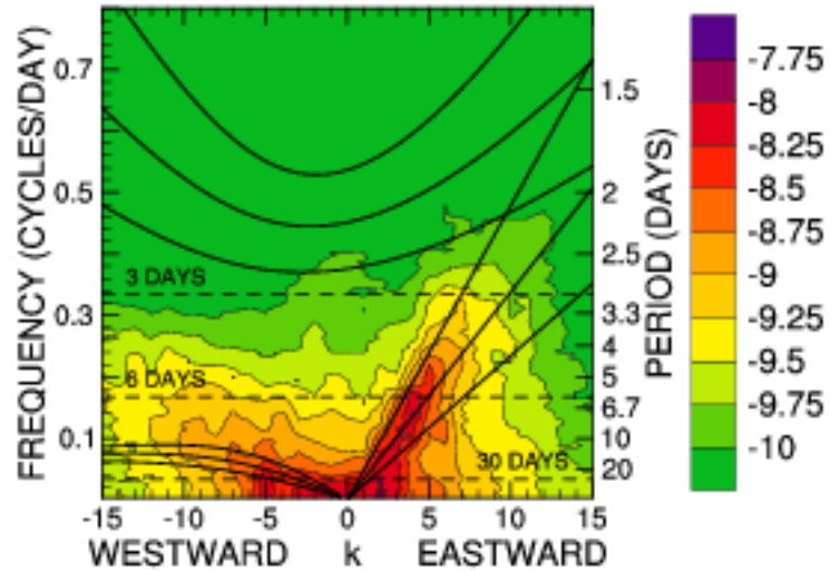
CONTROL SYMMETRIC CGAM
