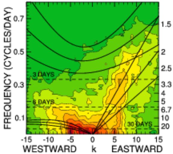
QOBS SYMMETRIC NCAR
