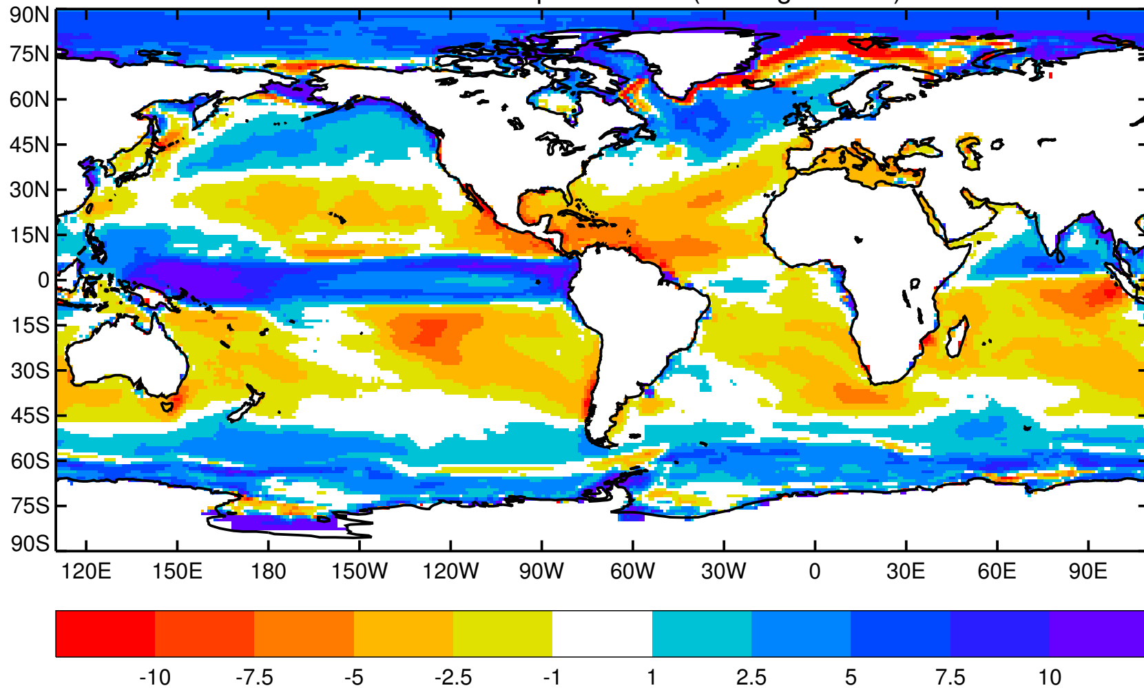
FAFMIP water flux perturbation ( 10^{-6} \text{ kg m}^{-2} \text{ s}^{-1} )
