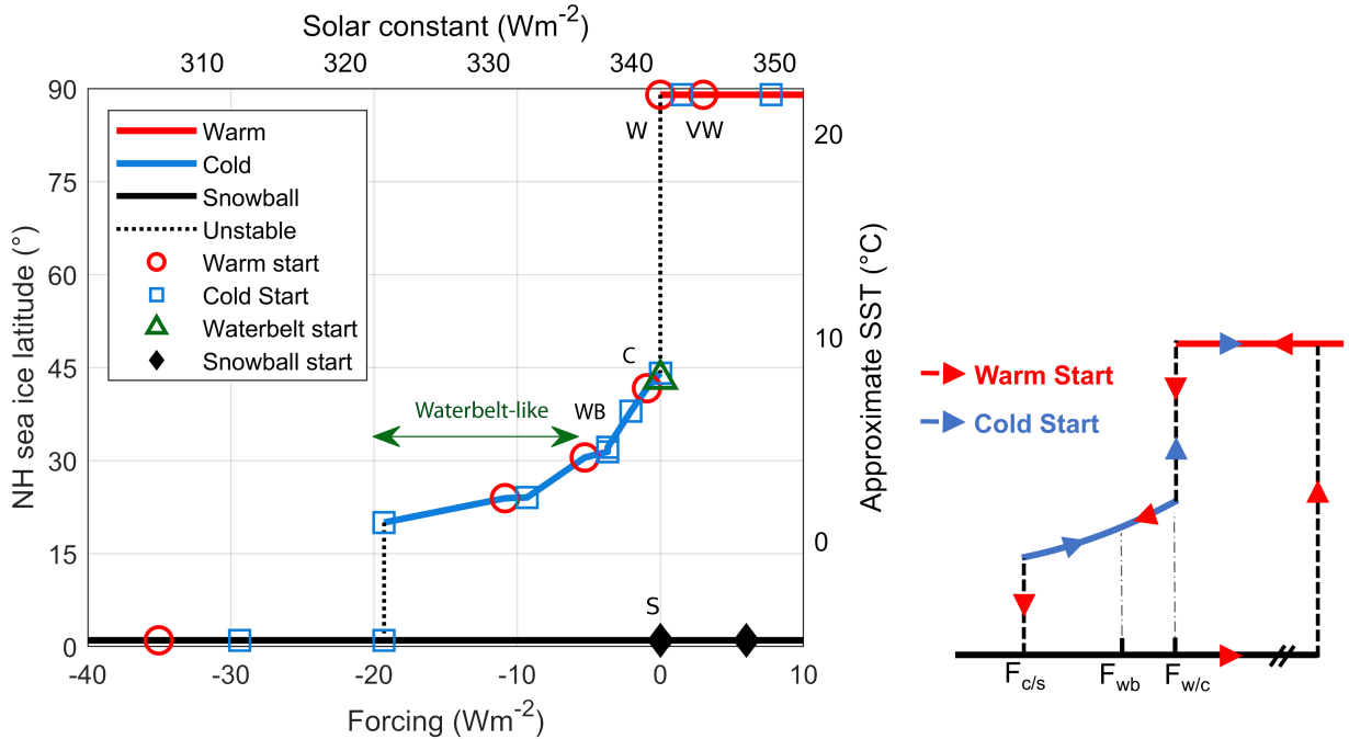
798 FIG. 3. (left) Bifurcation diagram of the climate model expressed in terms of the NH sea ice latitude (left 799 axis) versus the forcing F (bottom axis). F is calculated relative to the reference solar constant S_0 = 341.5 800 Wm^{-2} . The right axis indicates the approximate global mean SST and the top axis shows the solar constant. The 801 thick lines show the range of stable Warm (red), Cold (blue) and Snowball (black) states. The black dotted lines 802 indicate unstable NH sea ice latitudes. Each red circle, blue square, green triangle and black diamond shows the 803 equilibrated state of a simulation started from the Warm (W), Cold (C), Waterbelt (WB) and Snowball (S) states, 804 respectively. (right) Schematic plot (not to scale) representing the stable (solid) and unstable (dotted) branches 805 of the bifurcation diagram. The red arrows outline a possible path along the diagram starting from a Warm state 806 and the blue arrows shows a different path starting from a Cold state. F_{w/c} and F_{c/s} are transition thresholds 807 between the Warm/Cold and the Cold/Snowball equilibria respectively. F_{wb} ( = -5 Wm^{-2} ) is the forcing below 808 which the Cold states become Waterbelt-like.
