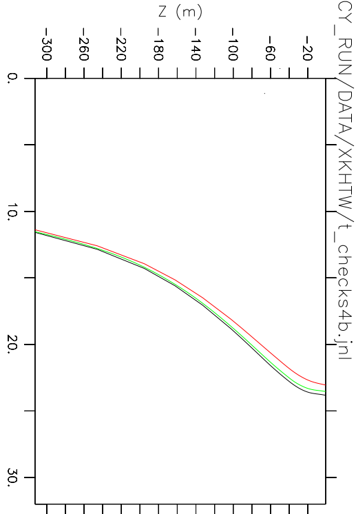
KPP Mean N(0:50N) Hem Temp/C
