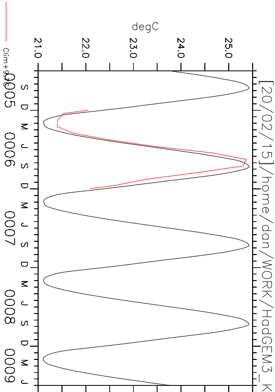
KPP Mean N Hem T at 10m
