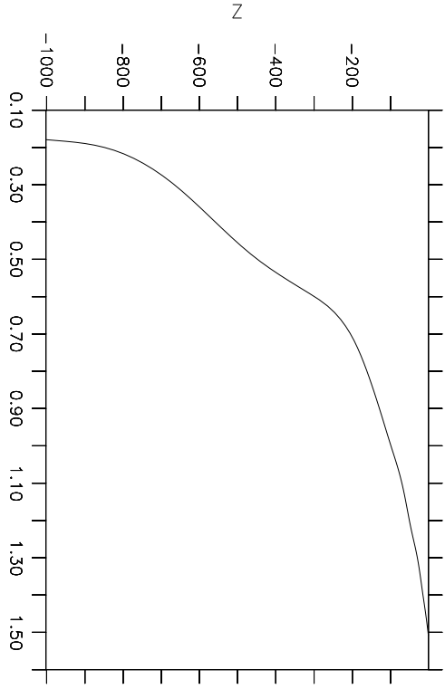
SD Salinity over year over area
