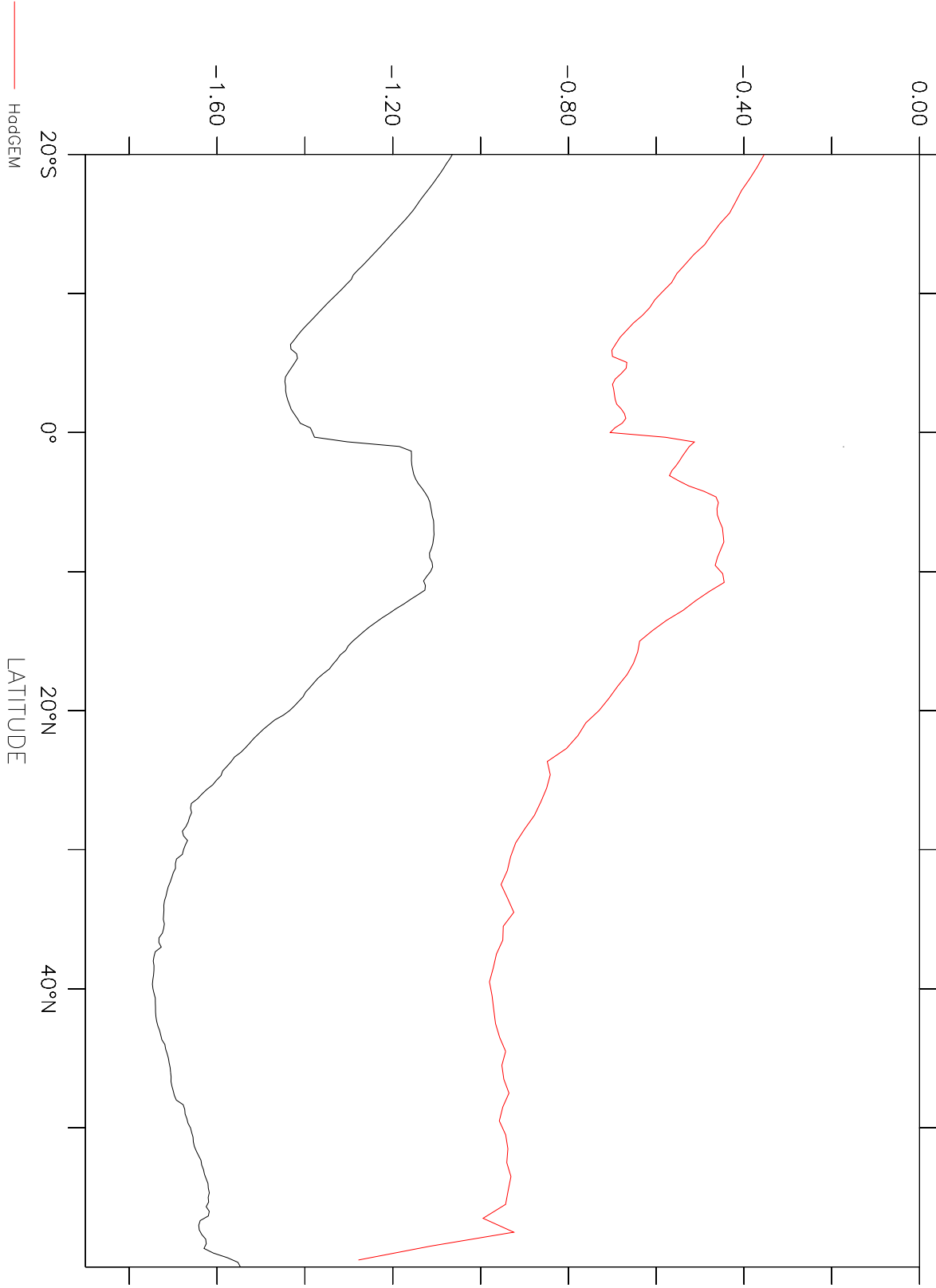
HiGEM Time Mean Depth Integrated V across Atl Basin/Sv
