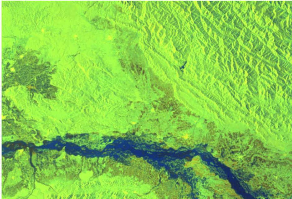
Raw Sentinel-1 satellite data on 12th of August 2017 over part of Brahmaputra river
