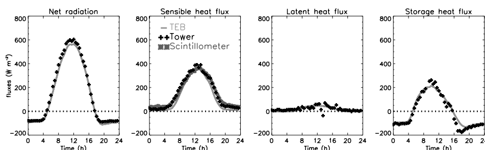
Figure 10. Comparison between observed and simulated surface energy balance fluxes in the city centre, averaged over 21 days. Black crosses – observed eddy covariance fluxes; continuous line – simulated fluxes using TEB, which are an average of the fluxes from roads, walls, roofs and natural surface cover. Grey stars in the turbulent sensible heat flux graph are calculated from the scintillometer data using the free-convection method (from Lemonsu et al., 2004).
